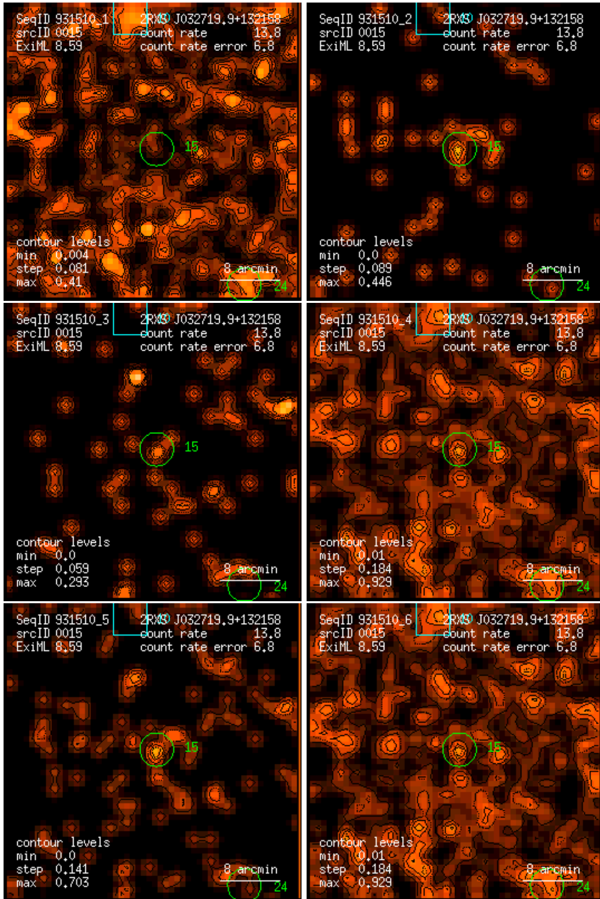
Figure 15: RASS 931510: detection 0015: band rate images, Gaussian filter: (1) PSPC channels 11 – 41, (2) 52 – 90, (3) 91 – 201, (4) 11 – 235, (5) 52 – 201, (6) 11 – 201. Broad band rates in counts/ks. Band rate contour levels in counts/ks/arcmin 2 .
