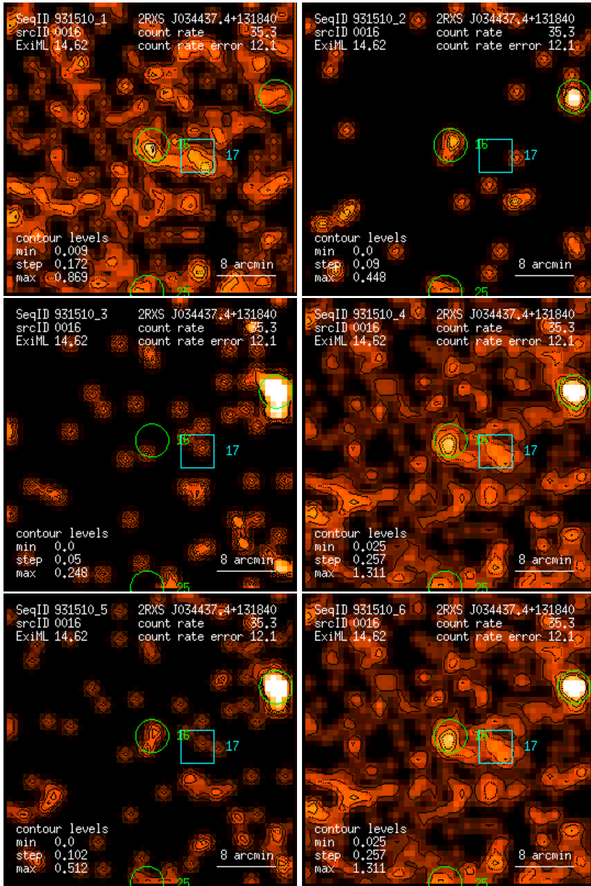
Figure 16: RASS 931510: detection 0016: band rate images, Gaussian filter: (1) PSPC channels 11 – 41, (2) 52 – 90, (3) 91 – 201, (4) 11 – 235, (5) 52 – 201, (6) 11 – 201. Broad band rates in counts/ks. Band rate contour levels in counts/ks/arcmin 2 .
