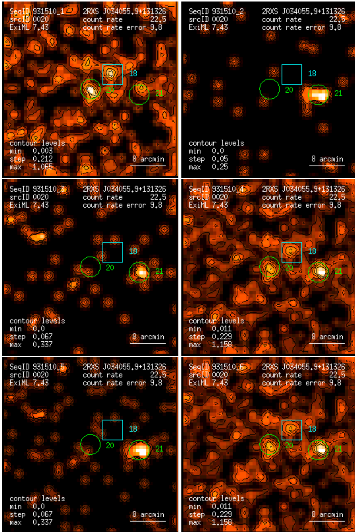
Figure 20: RASS 931510: detection 0020: band rate images, Gaussian filter: (1) PSPC channels 11 – 41, (2) 52 – 90, (3) 91 – 201, (4) 11 – 235, (5) 52 – 201, (6) 11 – 201. Broad band rates in counts/ks. Band rate contour levels in counts/ks/arcmin 2 .
