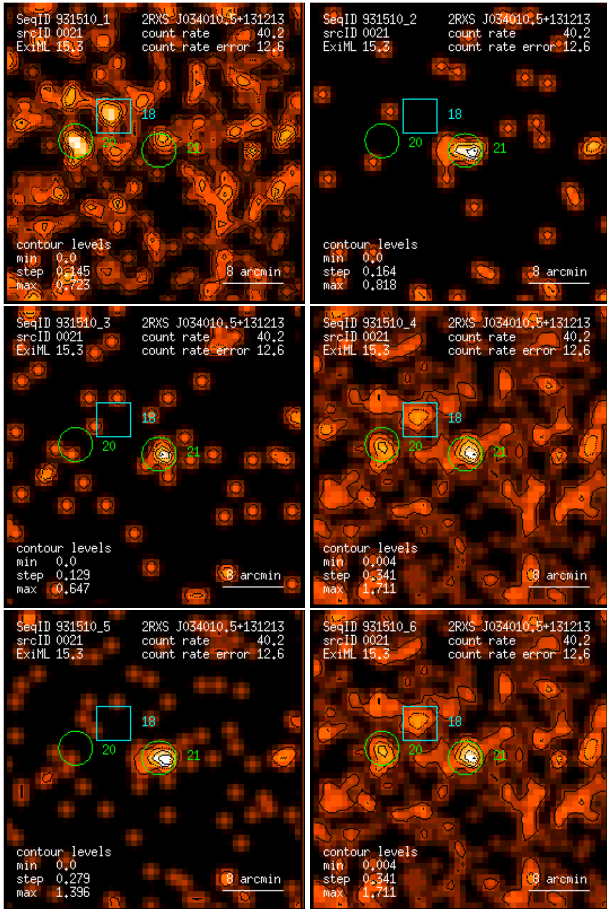
Figure 21: RASS 931510: detection 0021: band rate images, Gaussian filter: (1) PSPC channels 11 – 41, (2) 52 – 90, (3) 91 – 201, (4) 11 – 235, (5) 52 – 201, (6) 11 – 201. Broad band rates in counts/ks. Band rate contour levels in counts/ks/arcmin 2 .
