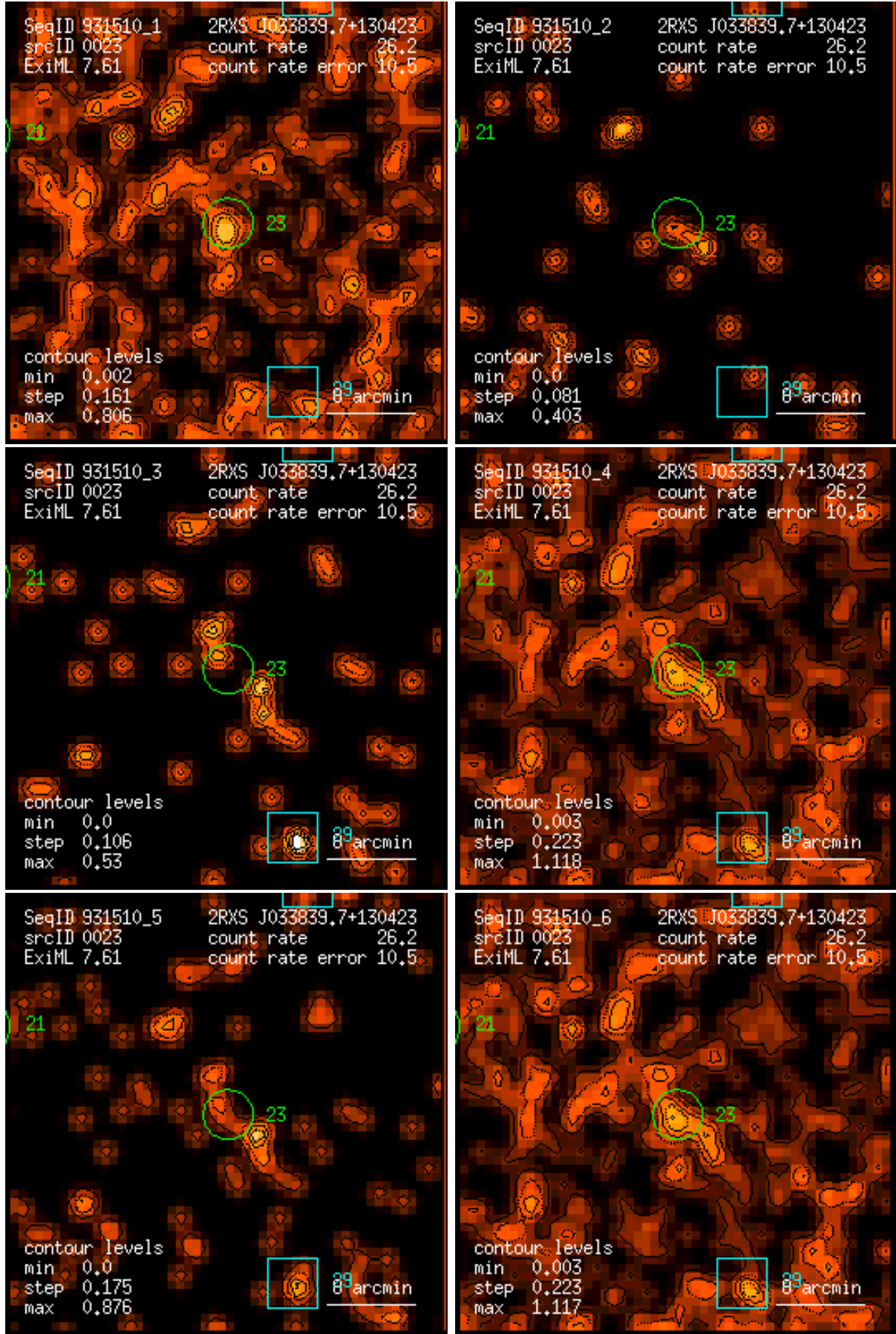
Figure 23: RASS 931510: detection 0023: band rate images, Gaussian filter: (1) PSPC channels 11 – 41, (2) 52 – 90, (3) 91 – 201, (4) 11 – 235, (5) 52 – 201, (6) 11 – 201. Broad band rates in counts/ks. Band rate contour levels in counts/ks/arcmin 2 .
