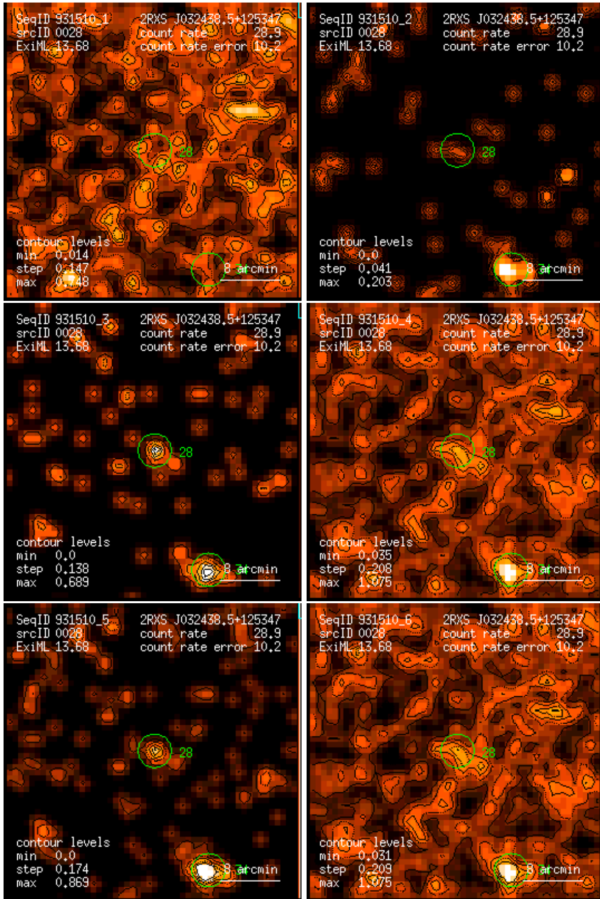
Figure 28: RASS 931510: detection 0028: band rate images, Gaussian filter: (1) PSPC channels 11 – 41, (2) 52 – 90, (3) 91 – 201, (4) 11 – 235, (5) 52 – 201, (6) 11 – 201. Broad band rates in counts/ks. Band rate contour levels in counts/ks/arcmin 2 .
