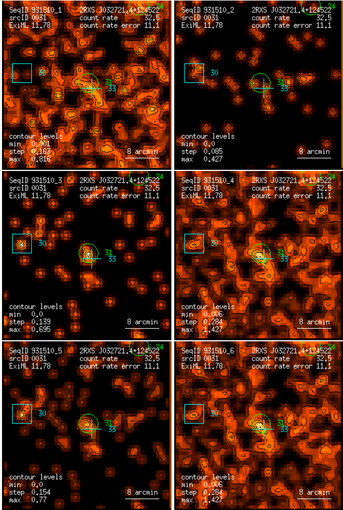
Figure 31: RASS 931510: detection 0031: band rate images, Gaussian filter: (1) PSPC channels 11 – 41, (2) 52 – 90, (3) 91 – 201, (4) 11 – 235, (5) 52 – 201, (6) 11 – 201. Broad band rates in counts/ks. Band rate contour levels in counts/ks/arcmin 2 .
