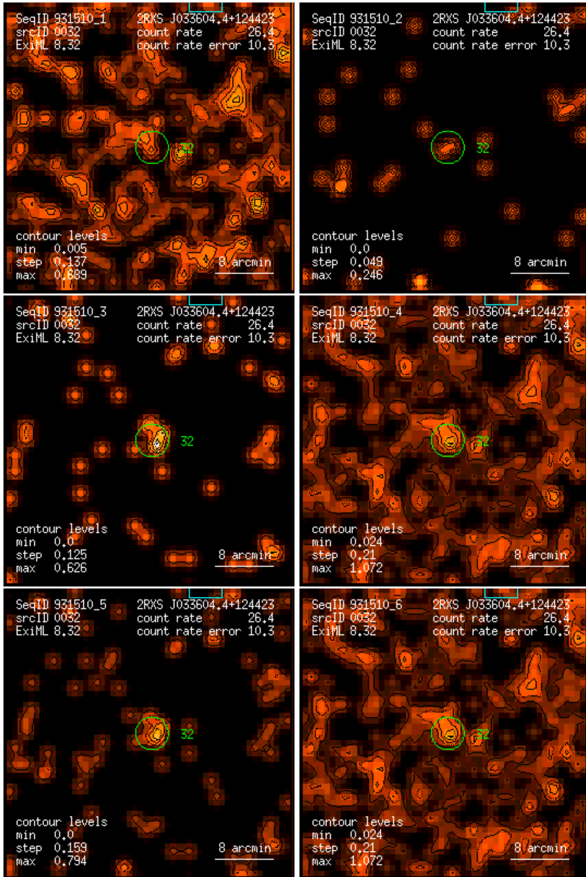
Figure 32: RASS 931510: detection 0032: band rate images, Gaussian filter: (1) PSPC channels 11 – 41, (2) 52 – 90, (3) 91 – 201, (4) 11 – 235, (5) 52 – 201, (6) 11 – 201. Broad band rates in counts/ks. Band rate contour levels in counts/ks/arcmin 2 .
