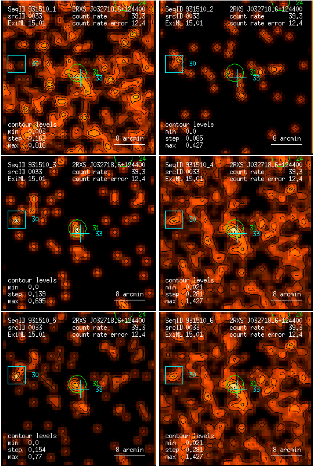
Figure 33: RASS 931510: detection 0033: band rate images, Gaussian filter: (1) PSPC channels 11 – 41, (2) 52 – 90, (3) 91 – 201, (4) 11 – 235, (5) 52 – 201, (6) 11 – 201. Broad band rates in counts/ks. Band rate contour levels in counts/ks/arcmin 2 .
