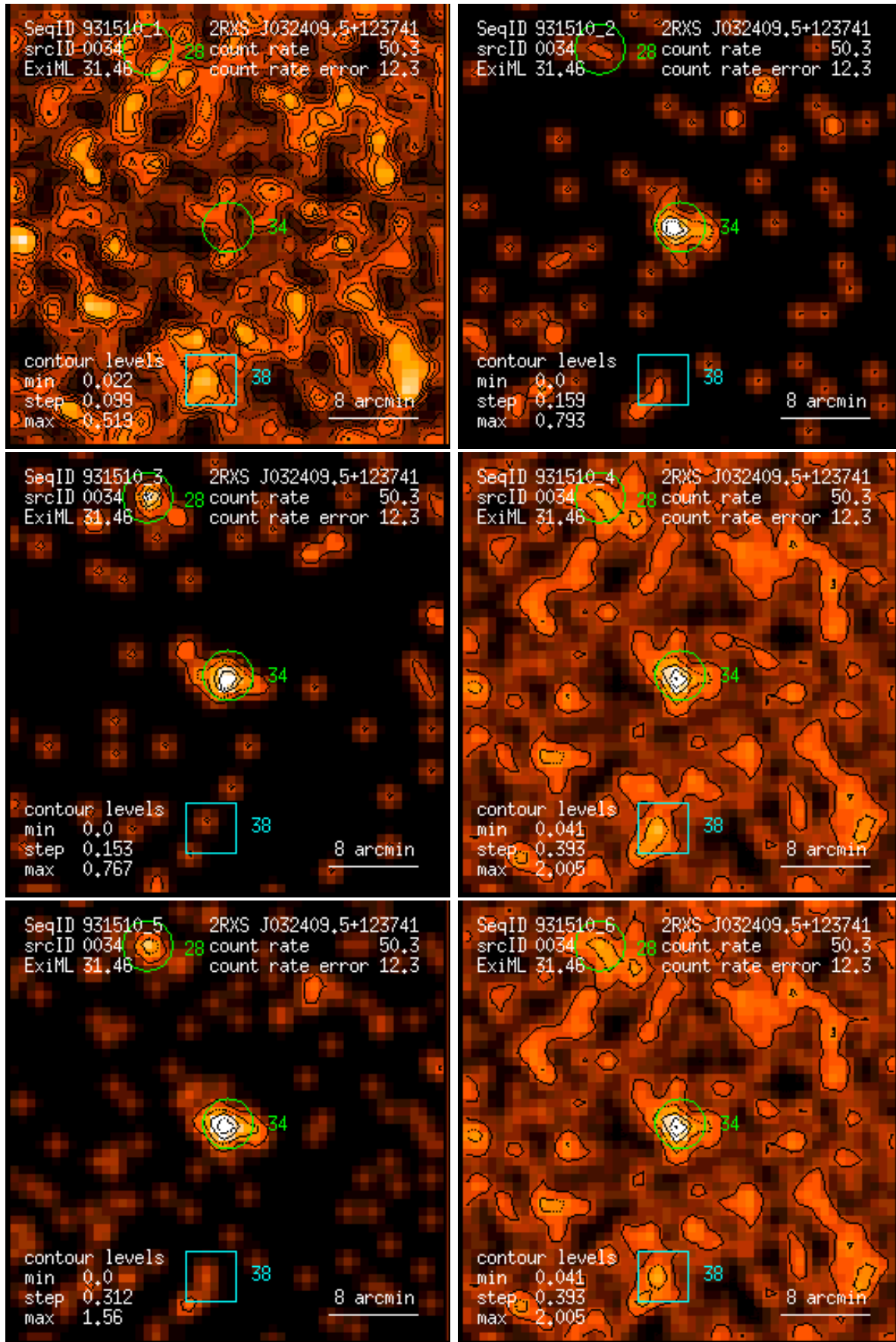
Figure 34: RASS 931510: detection 0034: band rate images, Gaussian filter: (1) PSPC channels 11 – 41, (2) 52 – 90, (3) 91 – 201, (4) 11 – 235, (5) 52 – 201, (6) 11 – 201. Broad band rates in counts/ks. Band rate contour levels in counts/ks/arcmin 2 .
