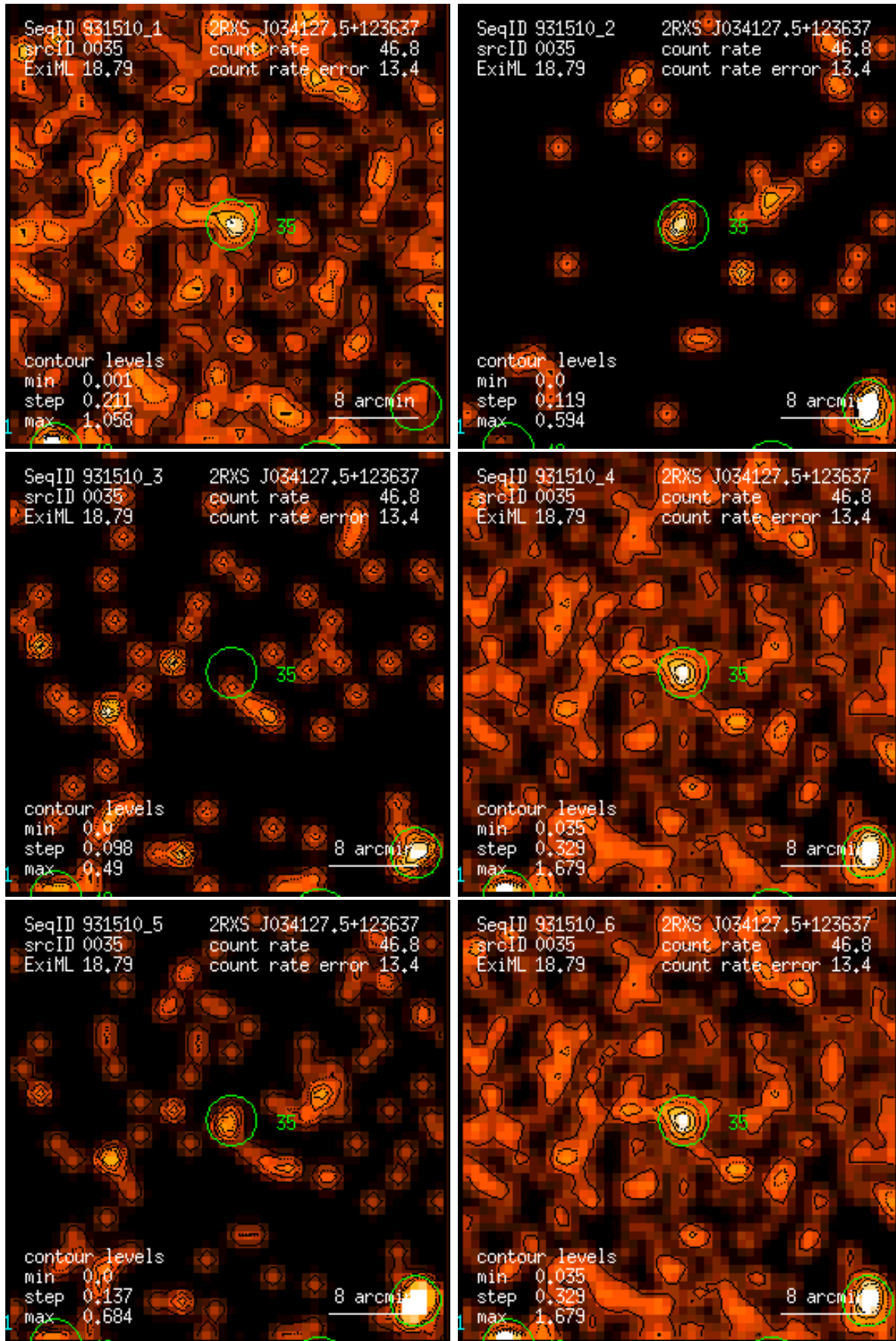
Figure 35: RASS 931510: detection 0035: band rate images, Gaussian filter: (1) PSPC channels 11 – 41, (2) 52 – 90, (3) 91 – 201, (4) 11 – 235, (5) 52 – 201, (6) 11 – 201. Broad band rates in counts/ks. Band rate contour levels in counts/ks/arcmin 2 .
