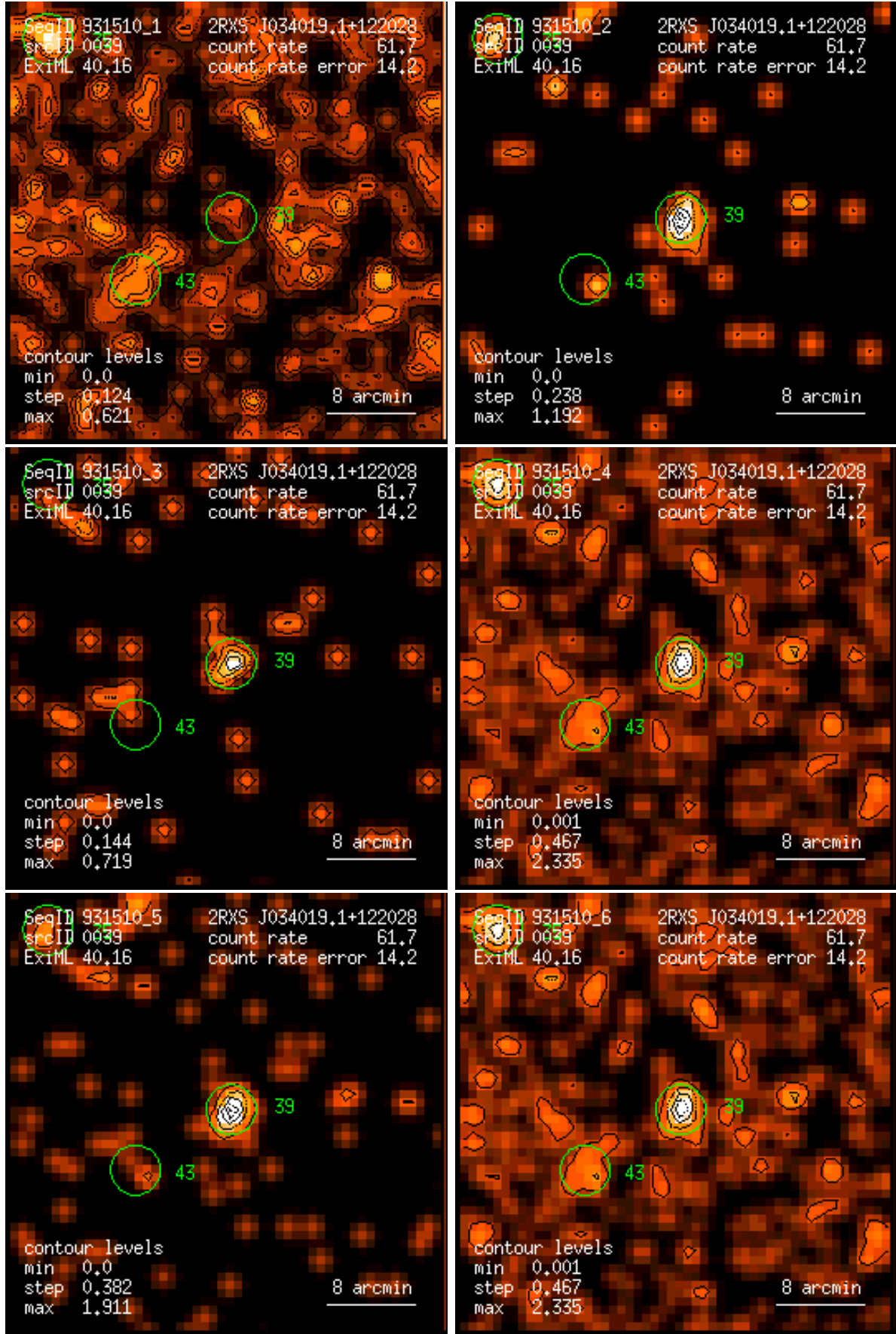
Figure 39: RASS 931510: detection 0039: band rate images, Gaussian filter: (1) PSPC channels 11 – 41, (2) 52 – 90, (3) 91 – 201, (4) 11 – 235, (5) 52 – 201, (6) 11 – 201. Broad band rates in counts/ks. Band rate contour levels in counts/ks/arcmin 2 .
