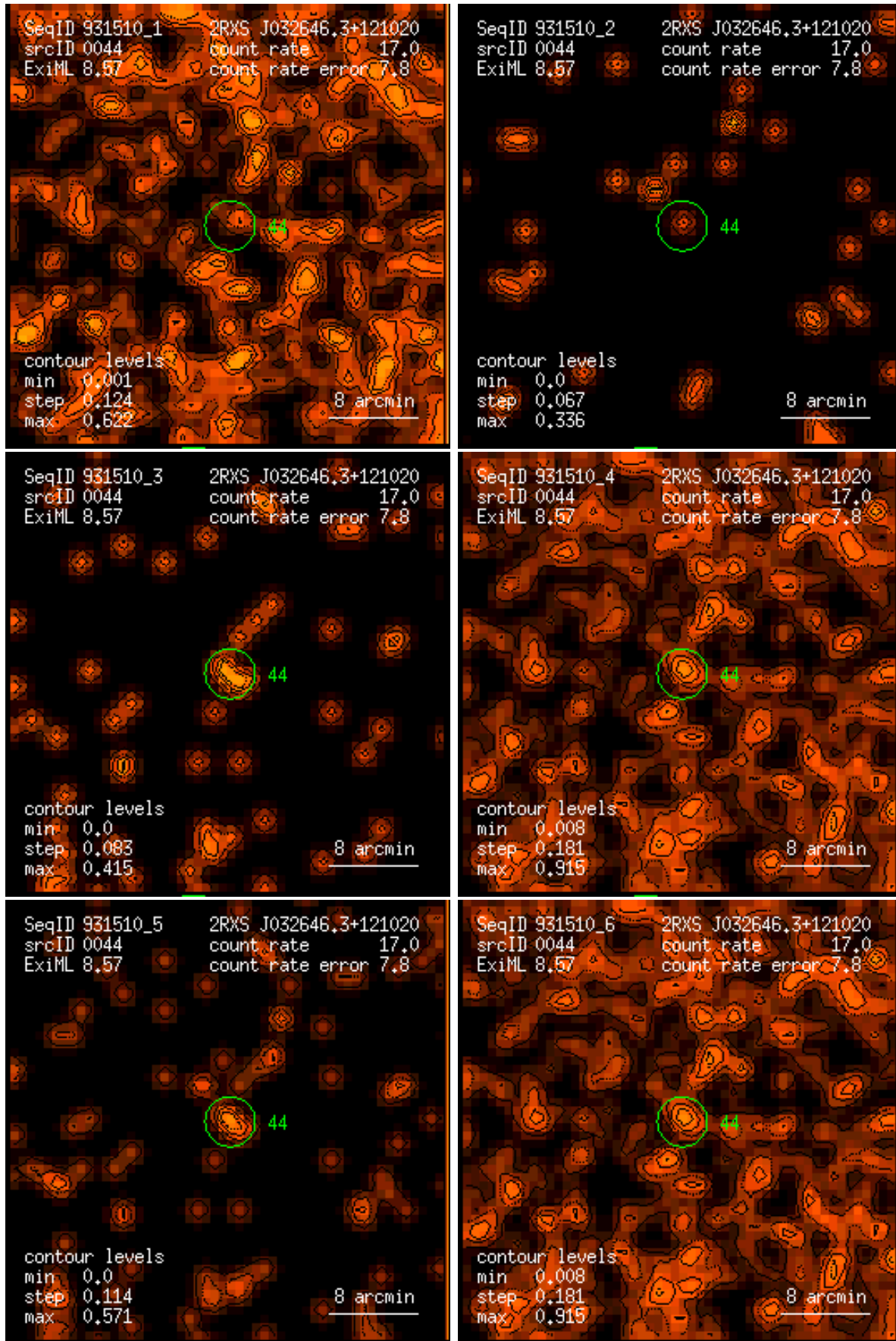
Figure 44: RASS 931510: detection 0044: band rate images, Gaussian filter: (1) PSPC channels 11 – 41, (2) 52 – 90, (3) 91 – 201, (4) 11 – 235, (5) 52 – 201, (6) 11 – 201. Broad band rates in counts/ks. Band rate contour levels in counts/ks/arcmin 2 .
