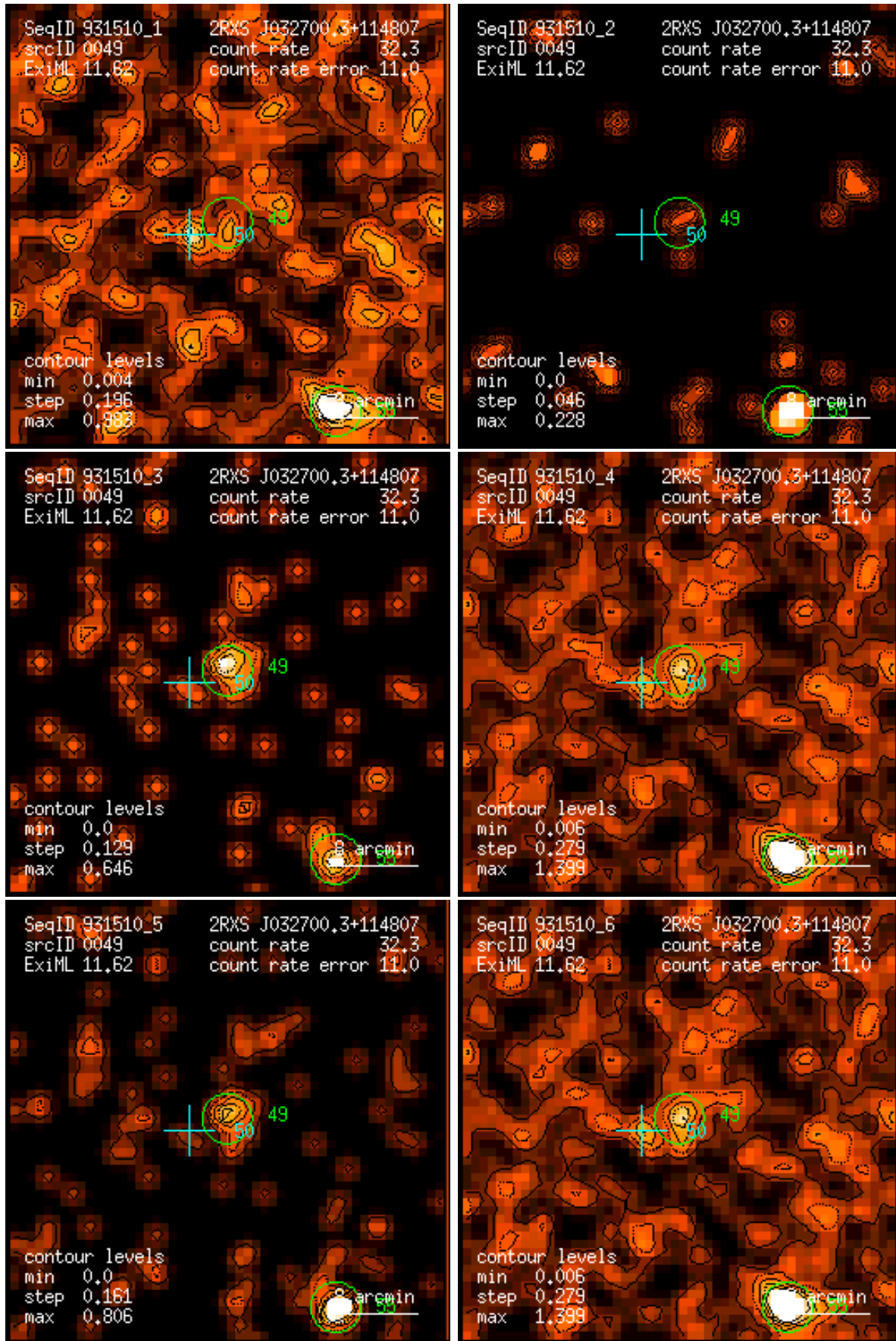
Figure 49: RASS 931510: detection 0049: band rate images, Gaussian filter: (1) PSPC channels 11 – 41, (2) 52 – 90, (3) 91 – 201, (4) 11 – 235, (5) 52 – 201, (6) 11 – 201. Broad band rates in counts/ks. Band rate contour levels in counts/ks/arcmin 2 .
