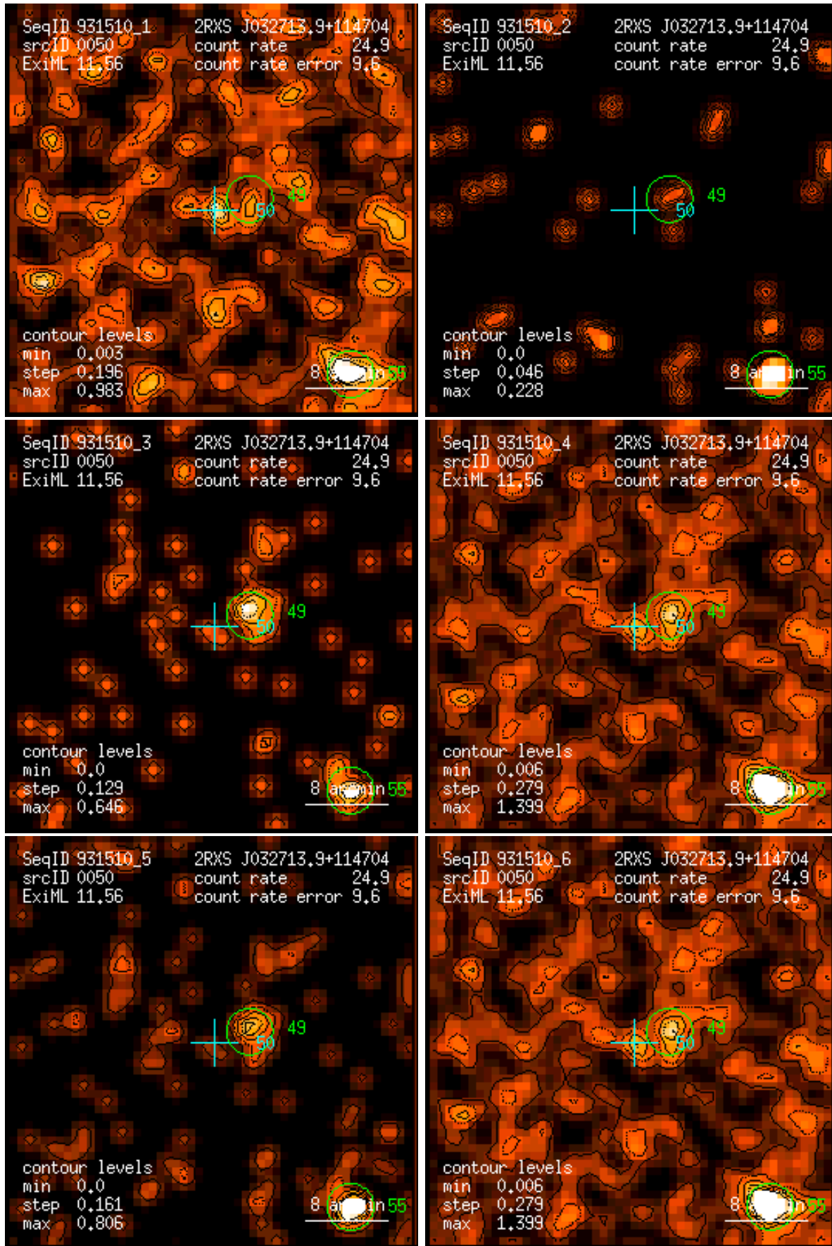
Figure 50: RASS 931510: detection 0050: band rate images, Gaussian filter: (1) PSPC channels 11 – 41, (2) 52 – 90, (3) 91 – 201, (4) 11 – 235, (5) 52 – 201, (6) 11 – 201. Broad band rates in counts/ks. Band rate contour levels in counts/ks/arcmin 2 .
