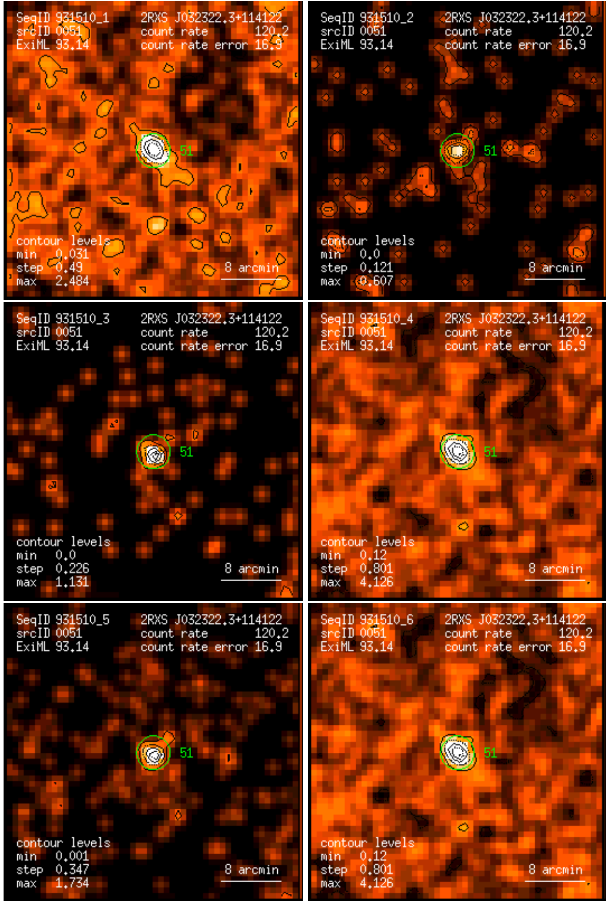
Figure 51: RASS 931510: detection 0051: band rate images, Gaussian filter: (1) PSPC channels 11 – 41, (2) 52 – 90, (3) 91 – 201, (4) 11 – 235, (5) 52 – 201, (6) 11 – 201. Broad band rates in counts/ks. Band rate contour levels in counts/ks/arcmin 2 .
