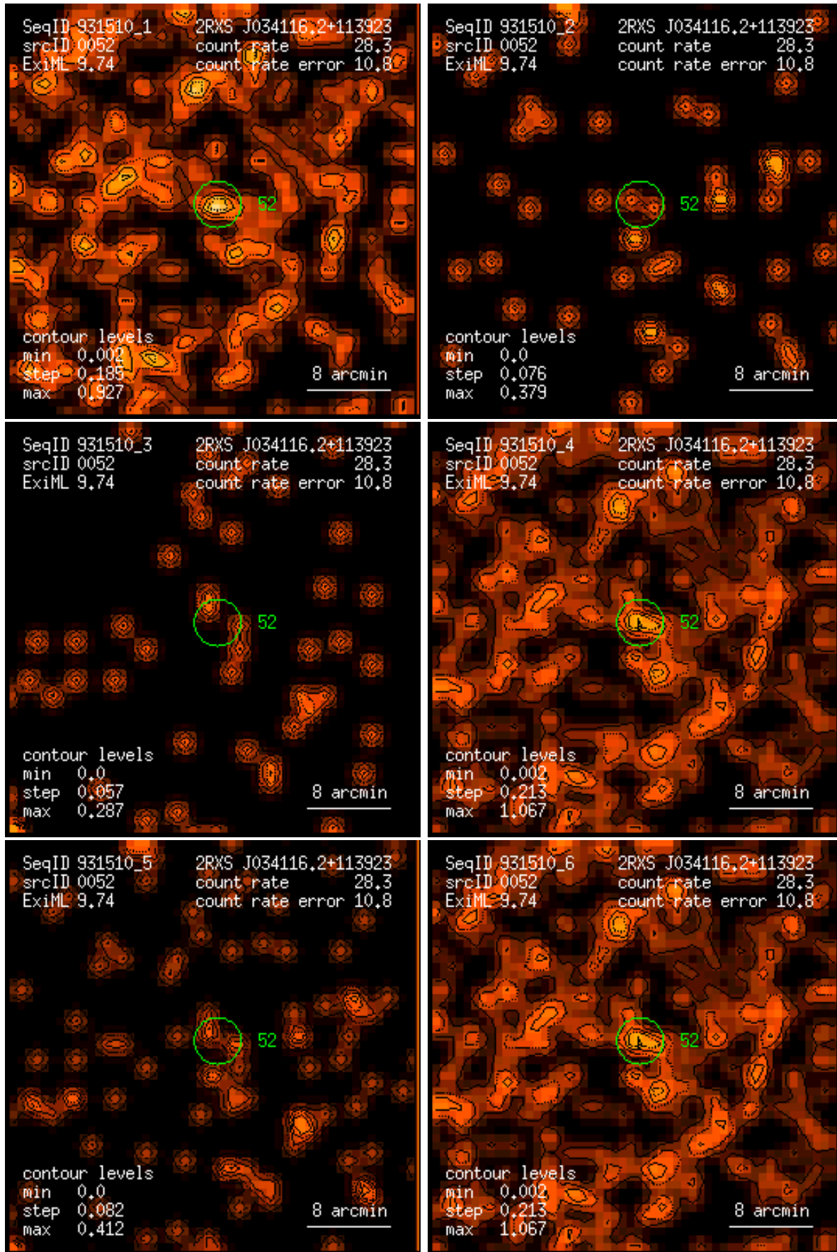
Figure 52: RASS 931510: detection 0052: band rate images, Gaussian filter: (1) PSPC channels 11 – 41, (2) 52 – 90, (3) 91 – 201, (4) 11 – 235, (5) 52 – 201, (6) 11 – 201. Broad band rates in counts/ks. Band rate contour levels in counts/ks/arcmin 2 .
