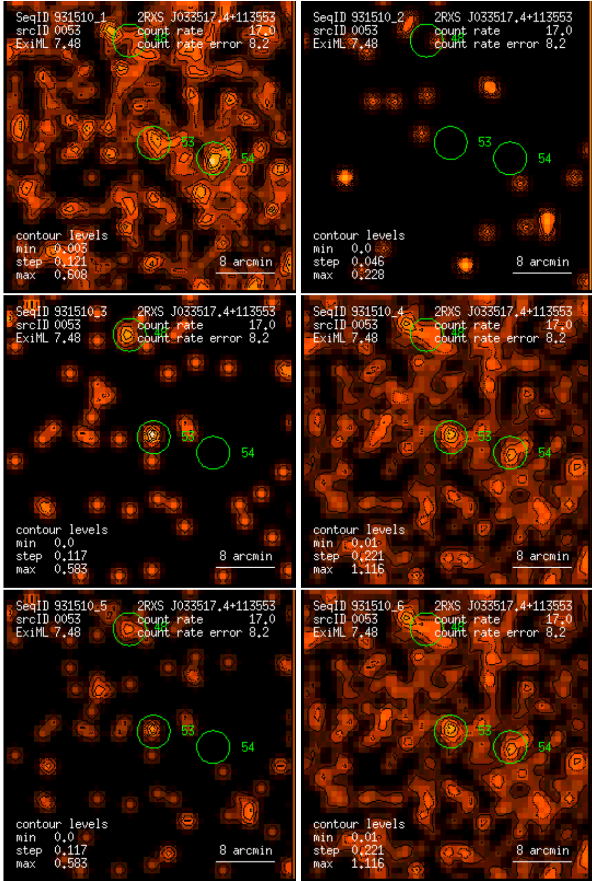
Figure 53: RASS 931510: detection 0053: band rate images, Gaussian filter: (1) PSPC channels 11 – 41, (2) 52 – 90, (3) 91 – 201, (4) 11 – 235, (5) 52 – 201, (6) 11 – 201. Broad band rates in counts/ks. Band rate contour levels in counts/ks/arcmin 2 .
