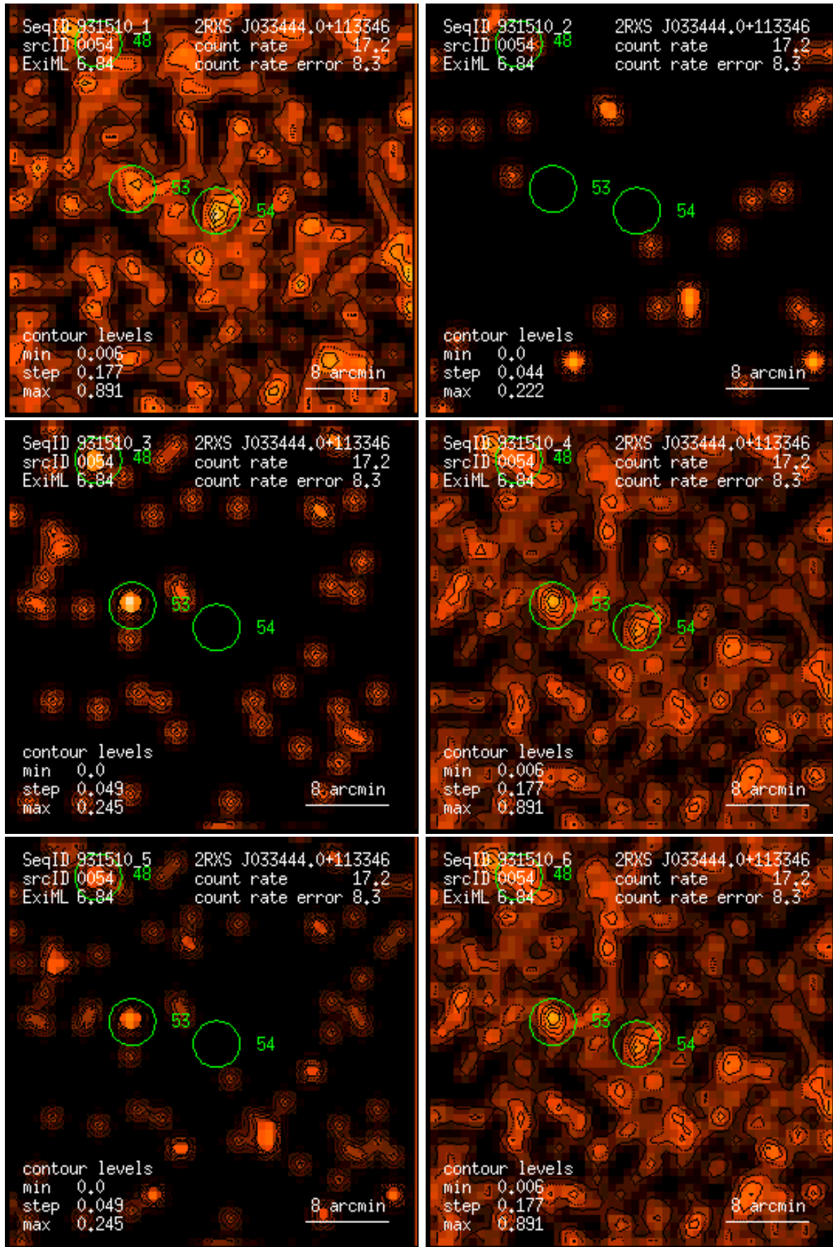
Figure 54: RASS 931510: detection 0054: band rate images, Gaussian filter: (1) PSPC channels 11 – 41, (2) 52 – 90, (3) 91 – 201, (4) 11 – 235, (5) 52 – 201, (6) 11 – 201. Broad band rates in counts/ks. Band rate contour levels in counts/ks/arcmin 2 .
