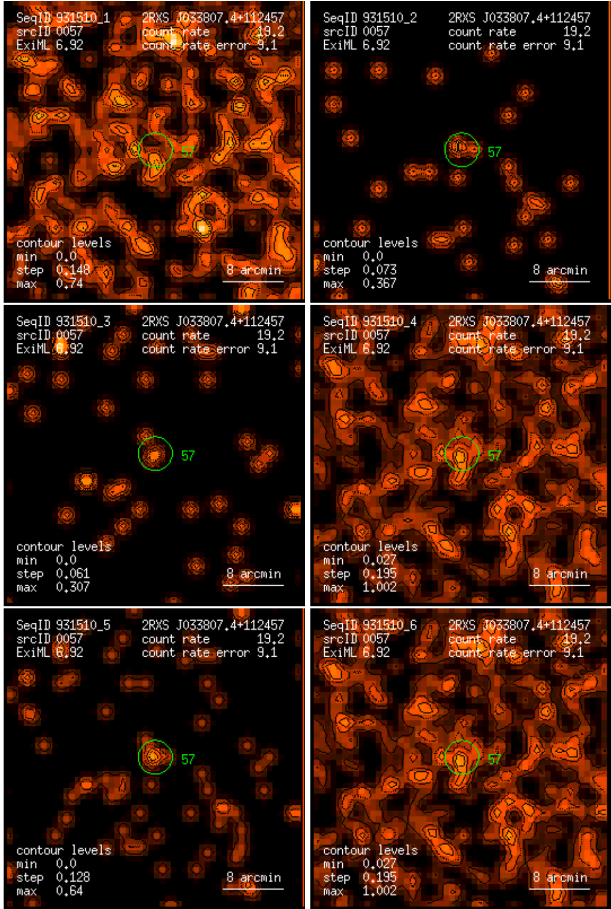
Figure 57: RASS 931510: detection 0057: band rate images, Gaussian filter: (1) PSPC channels 11 – 41, (2) 52 – 90, (3) 91 – 201, (4) 11 – 235, (5) 52 – 201, (6) 11 – 201. Broad band rates in counts/ks. Band rate contour levels in counts/ks/arcmin 2 .
