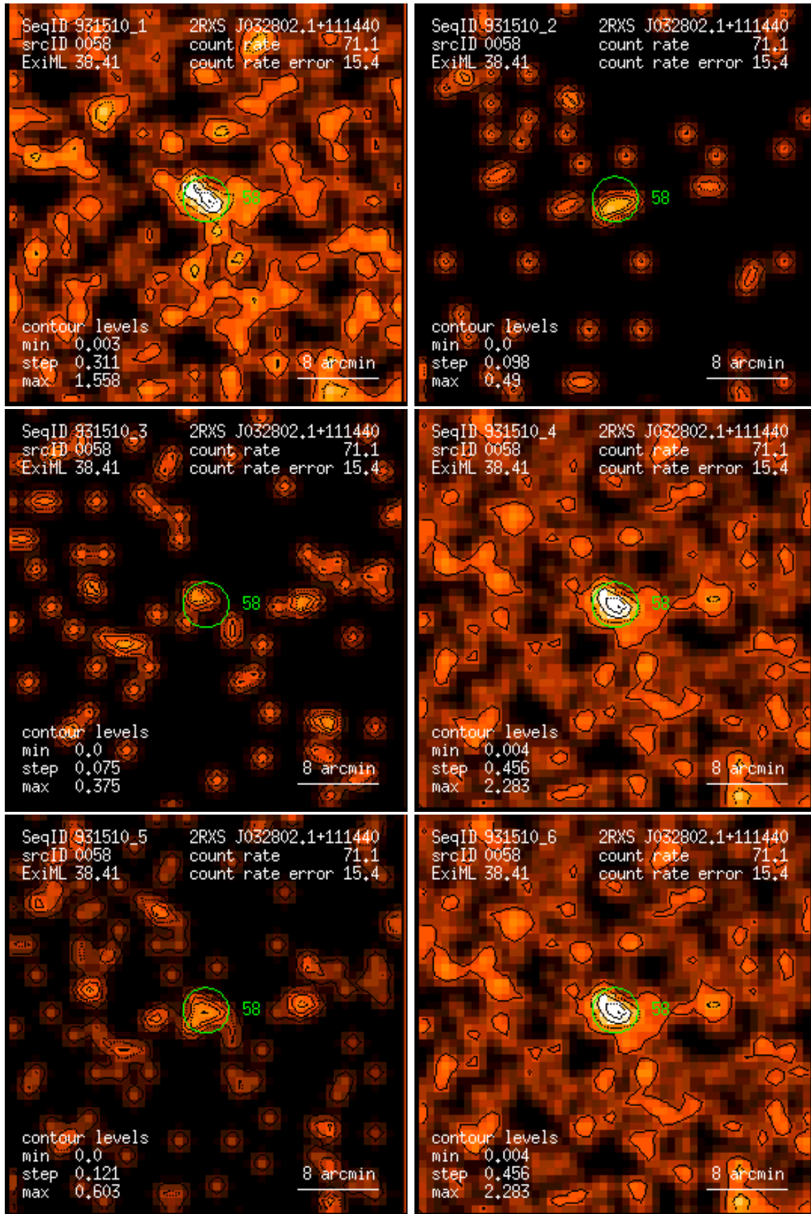
Figure 58: RASS 931510: detection 0058: band rate images, Gaussian filter: (1) PSPC channels 11 – 41, (2) 52 – 90, (3) 91 – 201, (4) 11 – 235, (5) 52 – 201, (6) 11 – 201. Broad band rates in counts/ks. Band rate contour levels in counts/ks/arcmin 2 .
