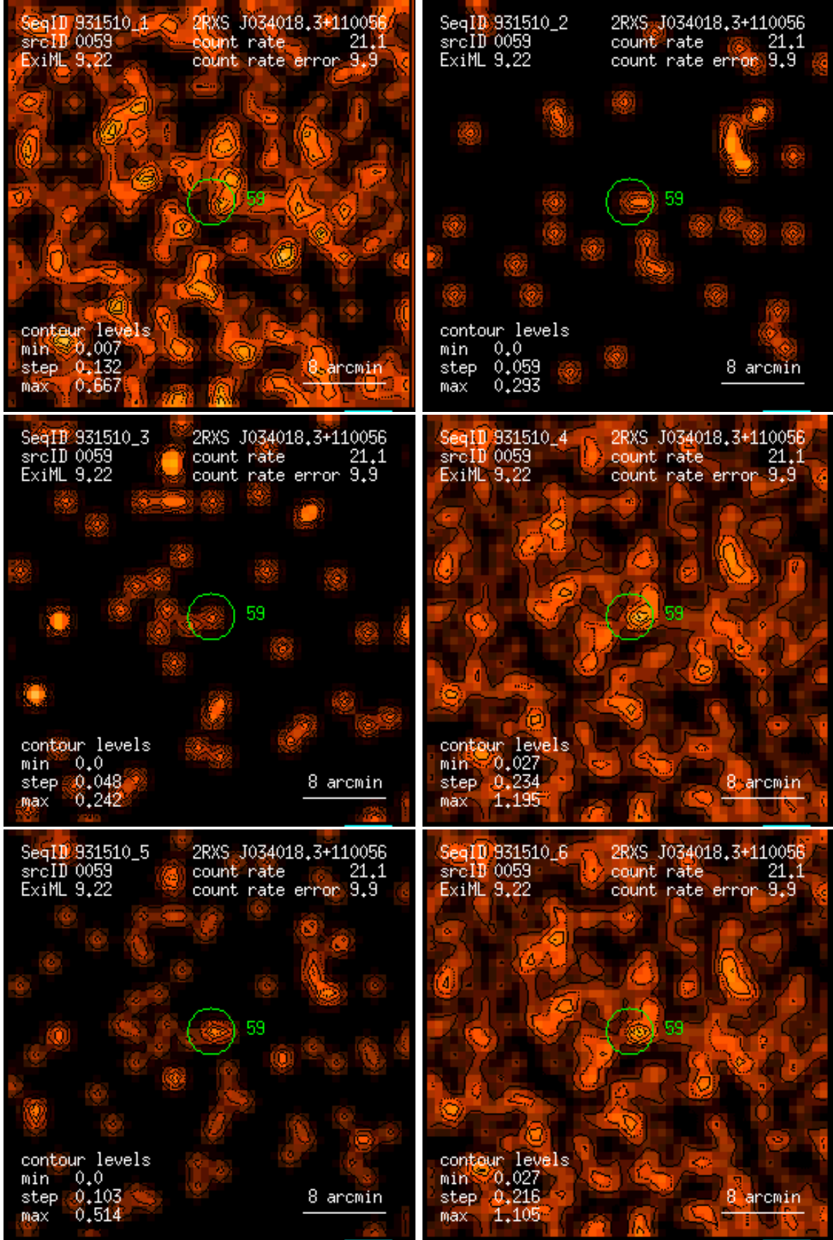
Figure 59: RASS 931510: detection 0059: band rate images, Gaussian filter: (1) PSPC channels 11 – 41, (2) 52 – 90, (3) 91 – 201, (4) 11 – 235, (5) 52 – 201, (6) 11 – 201. Broad band rates in counts/ks. Band rate contour levels in counts/ks/arcmin 2 .
