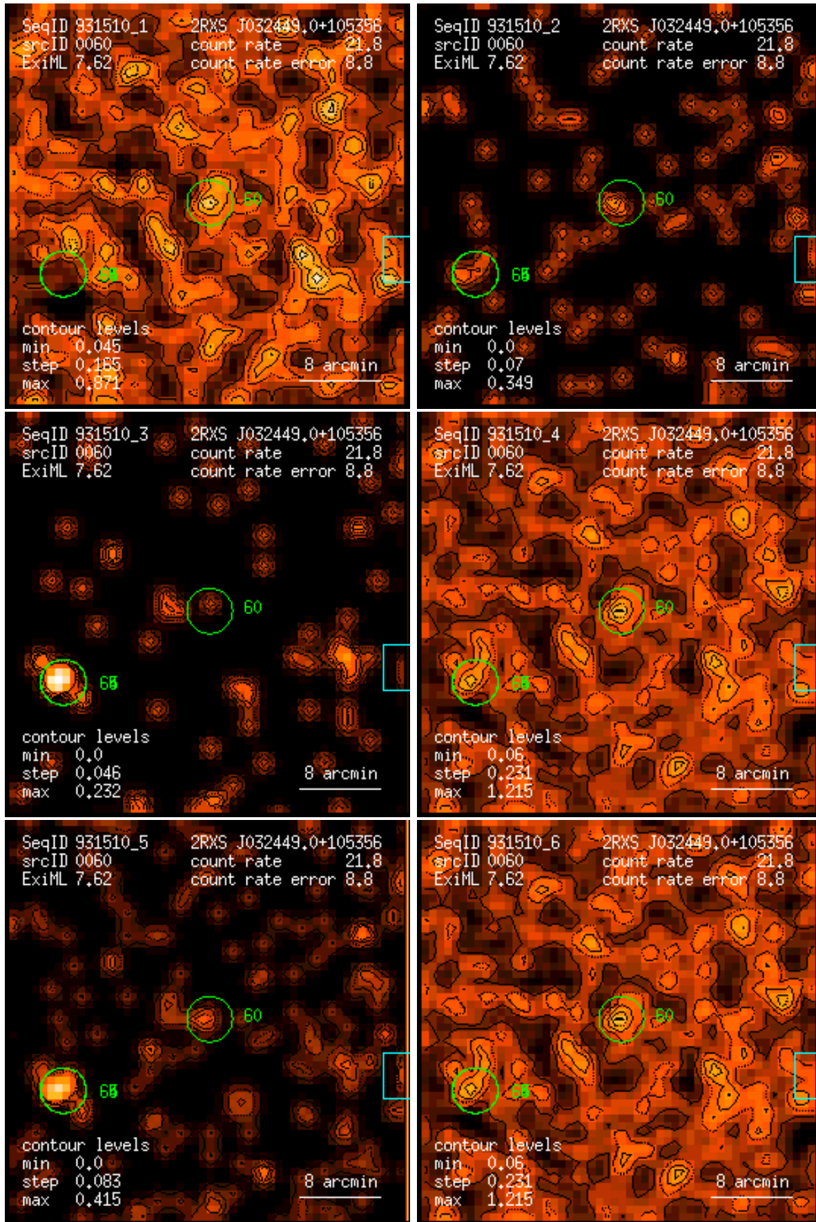
Figure 60: RASS 931510: detection 0060: band rate images, Gaussian filter: (1) PSPC channels 11 – 41, (2) 52 – 90, (3) 91 – 201, (4) 11 – 235, (5) 52 – 201, (6) 11 – 201. Broad band rates in counts/ks. Band rate contour levels in counts/ks/arcmin 2 .
