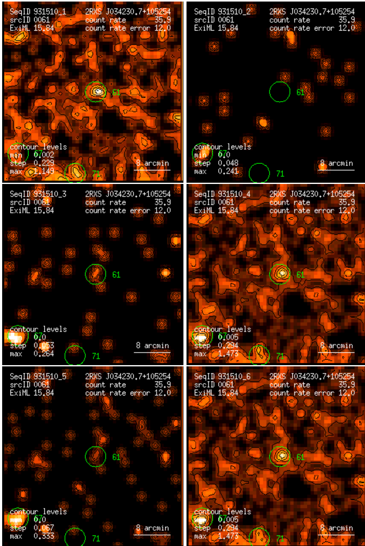
Figure 61: RASS 931510: detection 0061: band rate images, Gaussian filter: (1) PSPC channels 11 – 41, (2) 52 – 90, (3) 91 – 201, (4) 11 – 235, (5) 52 – 201, (6) 11 – 201. Broad band rates in counts/ks. Band rate contour levels in counts/ks/arcmin 2 .
