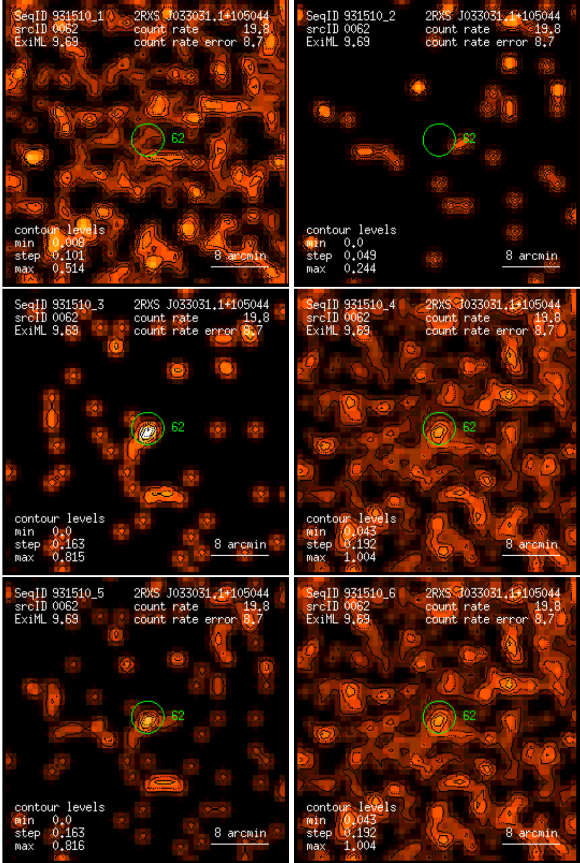
Figure 62: RASS 931510: detection 0062: band rate images, Gaussian filter: (1) PSPC channels 11 – 41, (2) 52 – 90, (3) 91 – 201, (4) 11 – 235, (5) 52 – 201, (6) 11 – 201. Broad band rates in counts/ks. Band rate contour levels in counts/ks/arcmin 2 .
