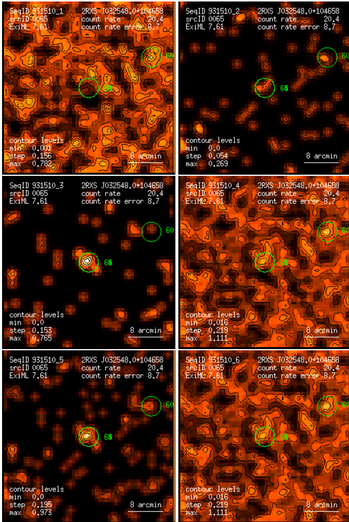
Figure 65: RASS 931510: detection 0065: band rate images, Gaussian filter: (1) PSPC channels 11 – 41, (2) 52 – 90, (3) 91 – 201, (4) 11 – 235, (5) 52 – 201, (6) 11 – 201. Broad band rates in counts/ks. Band rate contour levels in counts/ks/arcmin 2 .
