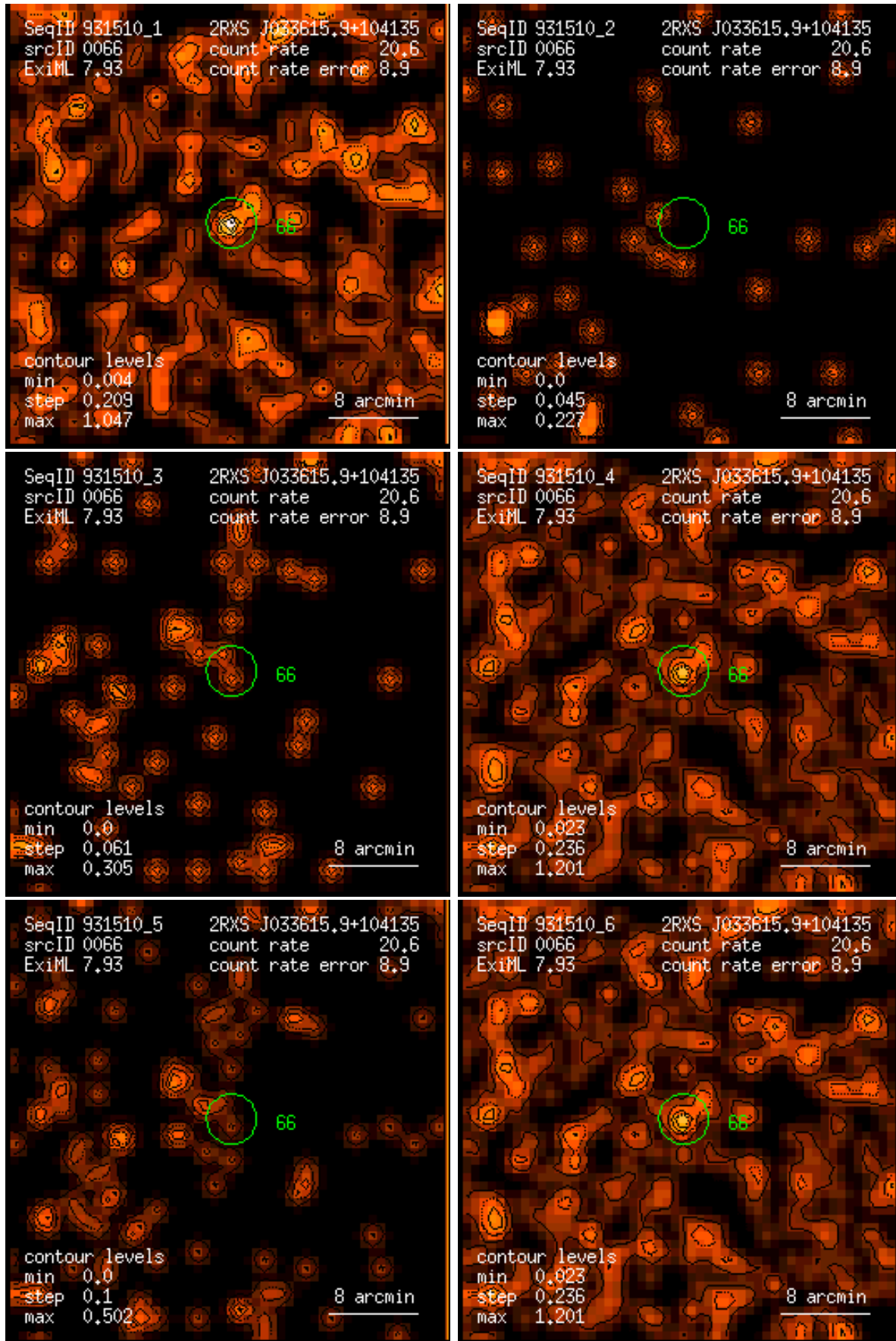
Figure 66: RASS 931510: detection 0066: band rate images, Gaussian filter: (1) PSPC channels 11 – 41, (2) 52 – 90, (3) 91 – 201, (4) 11 – 235, (5) 52 – 201, (6) 11 – 201. Broad band rates in counts/ks. Band rate contour levels in counts/ks/arcmin 2 .
