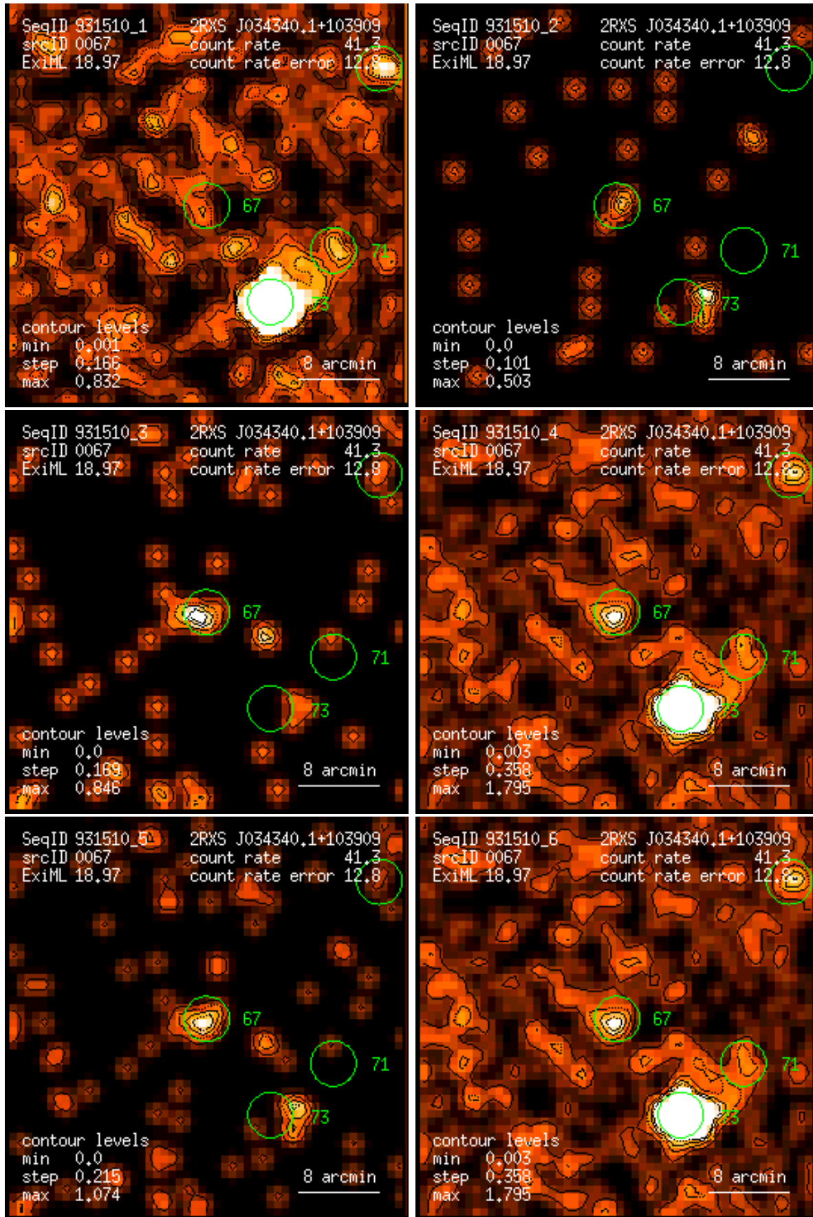
Figure 67: RASS 931510: detection 0067: band rate images, Gaussian filter: (1) PSPC channels 11 – 41, (2) 52 – 90, (3) 91 – 201, (4) 11 – 235, (5) 52 – 201, (6) 11 – 201. Broad band rates in counts/ks. Band rate contour levels in counts/ks/arcmin 2 .
