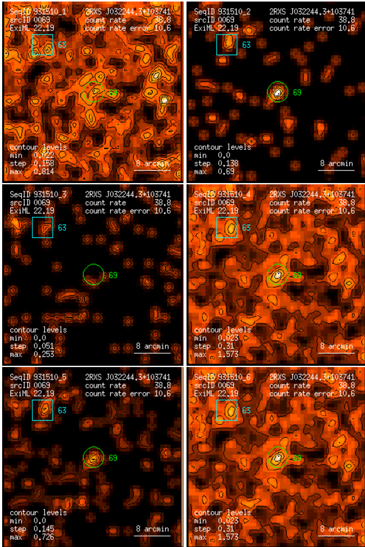
Figure 69: RASS 931510: detection 0069: band rate images, Gaussian filter: (1) PSPC channels 11 – 41, (2) 52 – 90, (3) 91 – 201, (4) 11 – 235, (5) 52 – 201, (6) 11 – 201. Broad band rates in counts/ks. Band rate contour levels in counts/ks/arcmin 2 .
