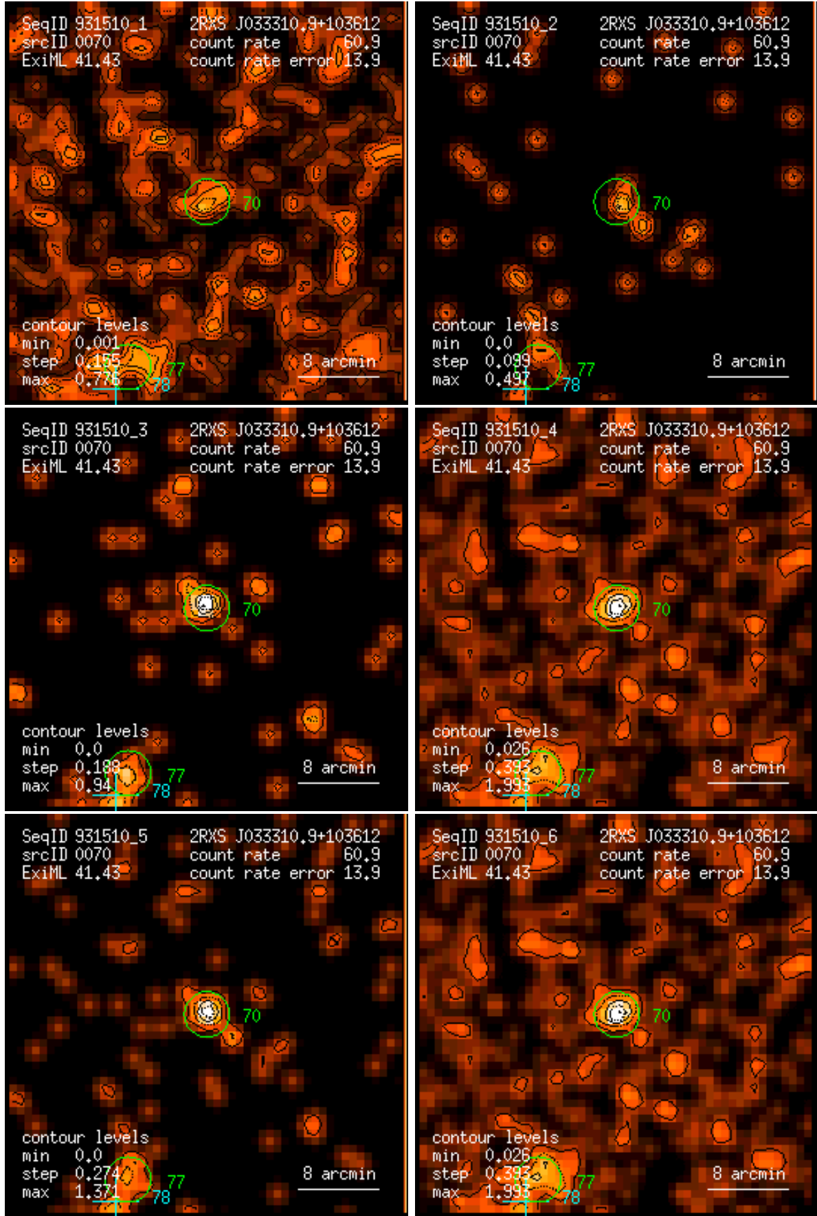
Figure 70: RASS 931510: detection 0070: band rate images, Gaussian filter: (1) PSPC channels 11 – 41, (2) 52 – 90, (3) 91 – 201, (4) 11 – 235, (5) 52 – 201, (6) 11 – 201. Broad band rates in counts/ks. Band rate contour levels in counts/ks/arcmin 2 .
