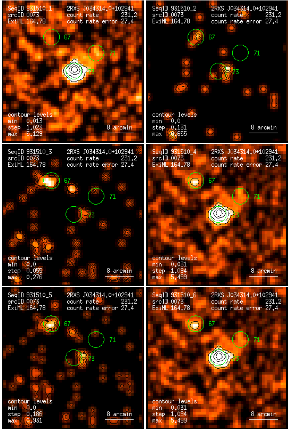
Figure 73: RASS 931510: detection 0073: band rate images, Gaussian filter: (1) PSPC channels 11 – 41, (2) 52 – 90, (3) 91 – 201, (4) 11 – 235, (5) 52 – 201, (6) 11 – 201. Broad band rates in counts/ks. Band rate contour levels in counts/ks/arcmin 2 .
