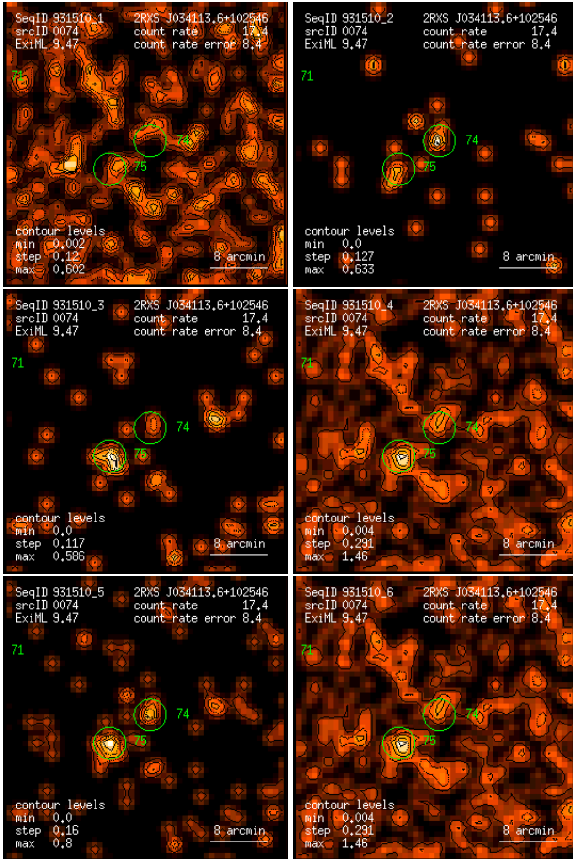
Figure 74: RASS 931510: detection 0074: band rate images, Gaussian filter: (1) PSPC channels 11 – 41, (2) 52 – 90, (3) 91 – 201, (4) 11 – 235, (5) 52 – 201, (6) 11 – 201. Broad band rates in counts/ks. Band rate contour levels in counts/ks/arcmin 2 .
