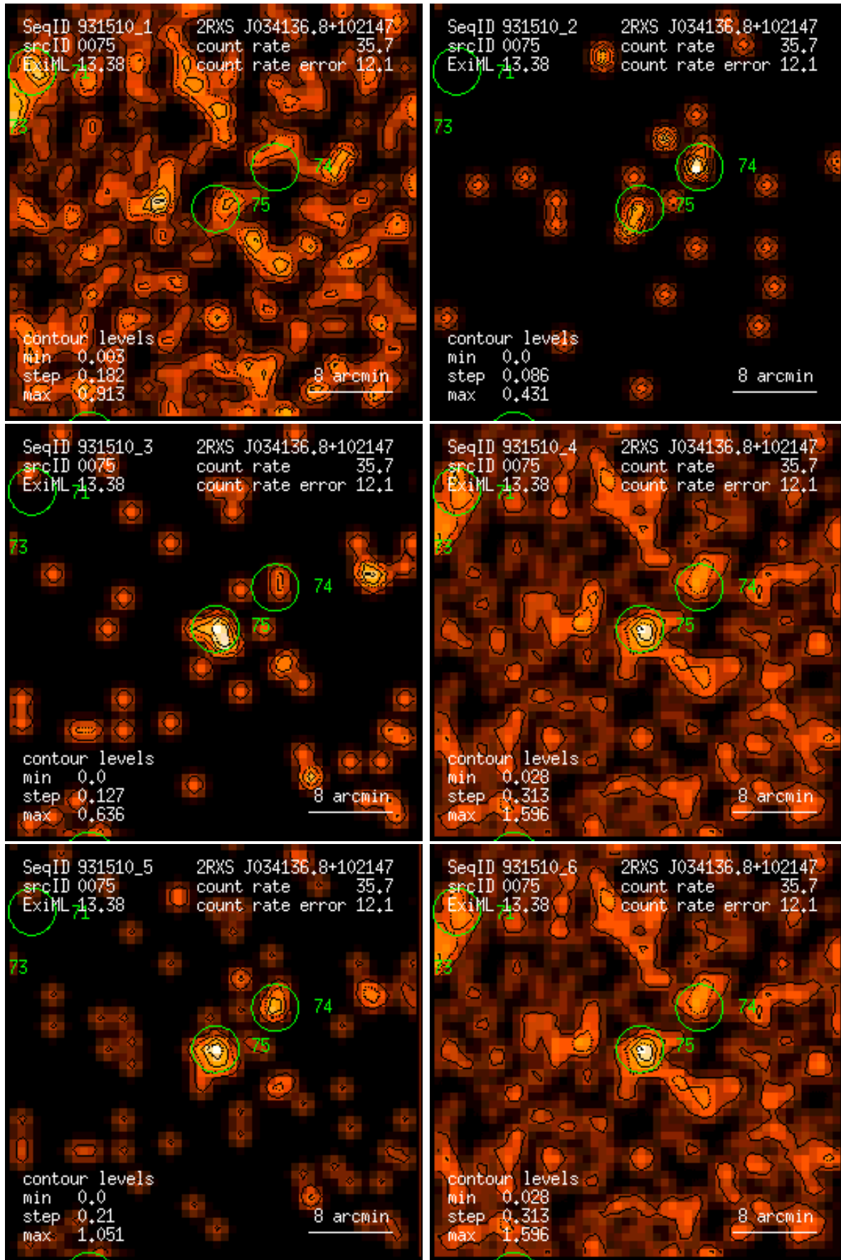
Figure 75: RASS 931510: detection 0075: band rate images, Gaussian filter: (1) PSPC channels 11 – 41, (2) 52 – 90, (3) 91 – 201, (4) 11 – 235, (5) 52 – 201, (6) 11 – 201. Broad band rates in counts/ks. Band rate contour levels in counts/ks/arcmin 2 .
