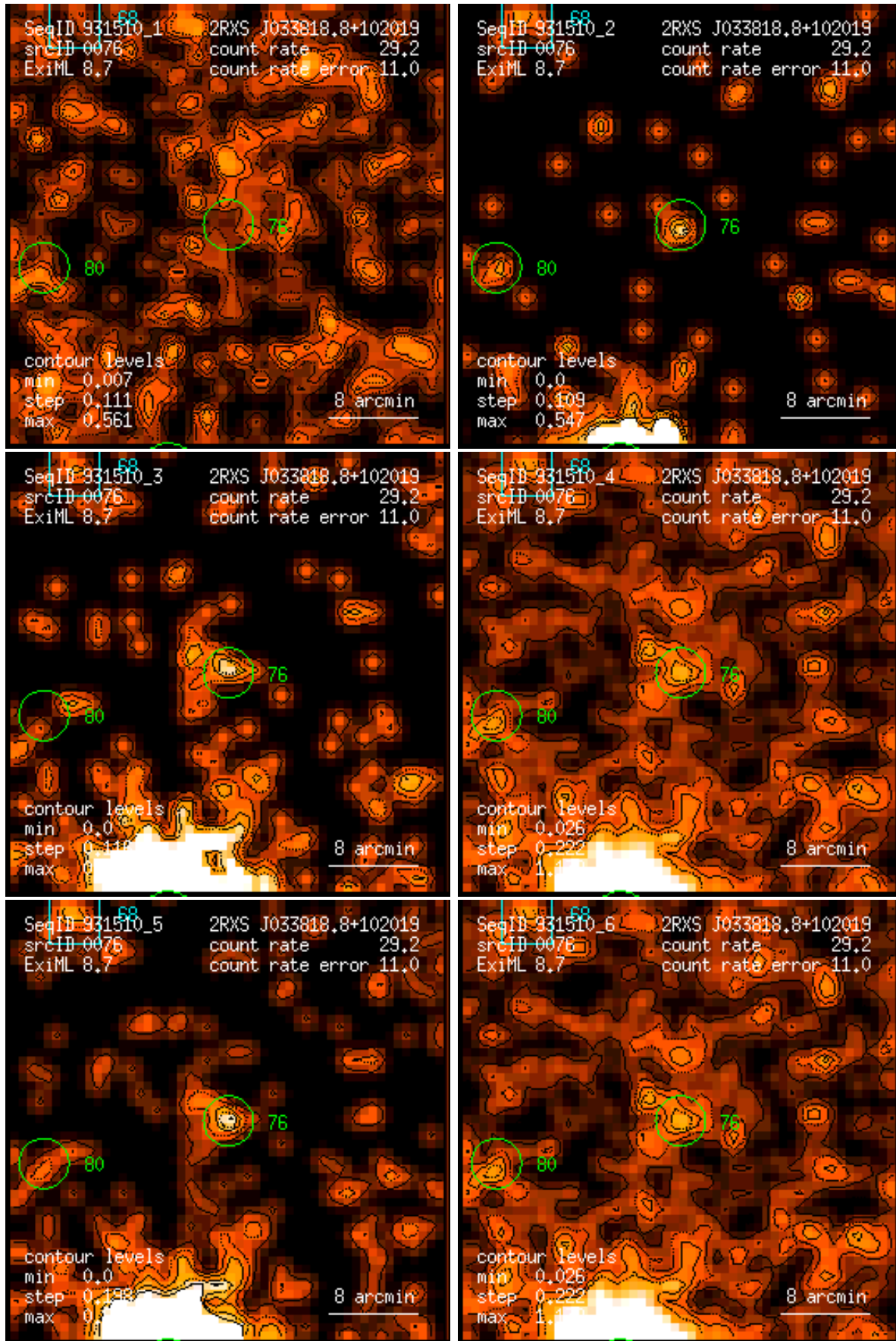
Figure 76: RASS 931510: detection 0076: band rate images, Gaussian filter: (1) PSPC channels 11 – 41, (2) 52 – 90, (3) 91 – 201, (4) 11 – 235, (5) 52 – 201, (6) 11 – 201. Broad band rates in counts/ks. Band rate contour levels in counts/ks/arcmin 2 .
