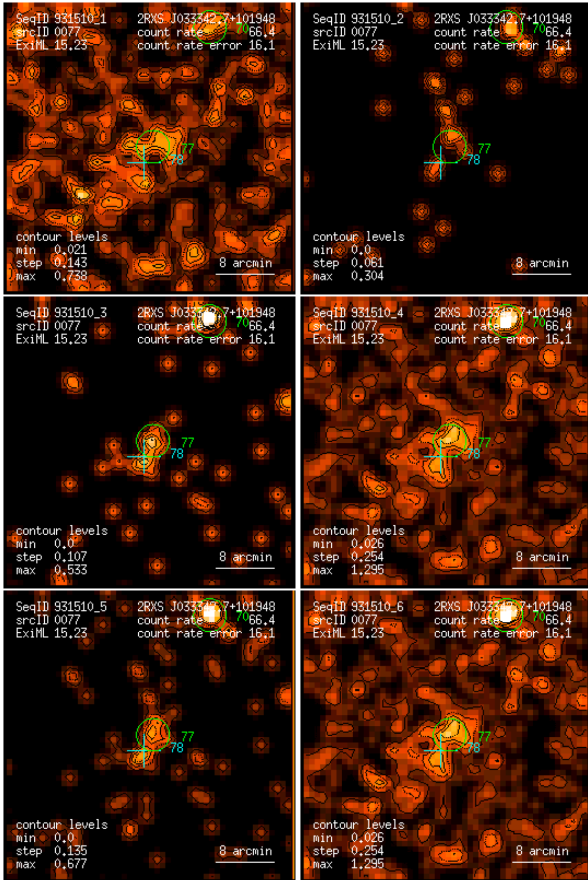
Figure 77: RASS 931510: detection 0077: band rate images, Gaussian filter: (1) PSPC channels 11 – 41, (2) 52 – 90, (3) 91 – 201, (4) 11 – 235, (5) 52 – 201, (6) 11 – 201. Broad band rates in counts/ks. Band rate contour levels in counts/ks/arcmin 2 .
