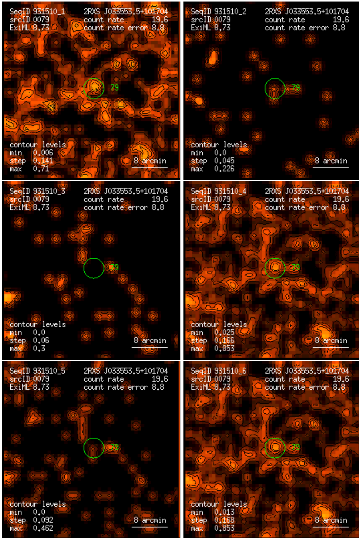
Figure 79: RASS 931510: detection 0079: band rate images, Gaussian filter: (1) PSPC channels 11 – 41, (2) 52 – 90, (3) 91 – 201, (4) 11 – 235, (5) 52 – 201, (6) 11 – 201. Broad band rates in counts/ks. Band rate contour levels in counts/ks/arcmin 2 .
