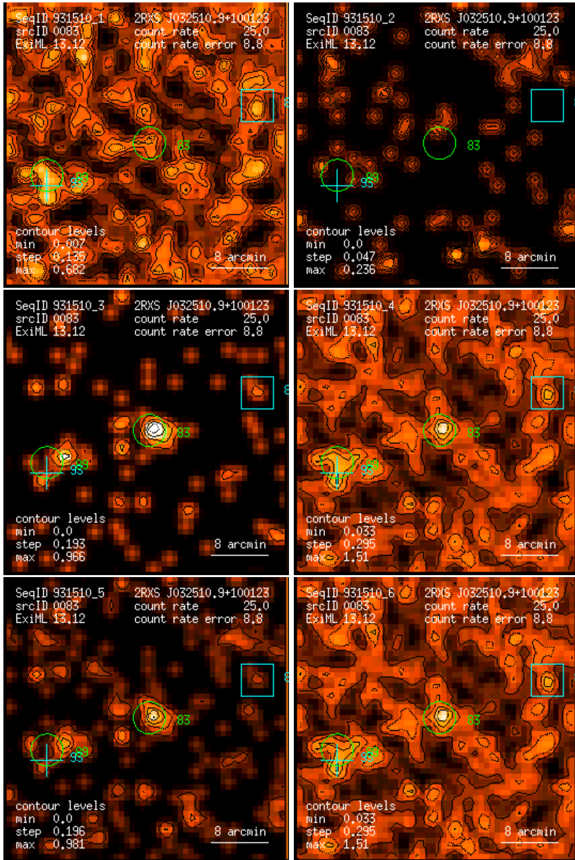
Figure 83: RASS 931510: detection 0083: band rate images, Gaussian filter: (1) PSPC channels 11 – 41, (2) 52 – 90, (3) 91 – 201, (4) 11 – 235, (5) 52 – 201, (6) 11 – 201. Broad band rates in counts/ks. Band rate contour levels in counts/ks/arcmin 2 .
