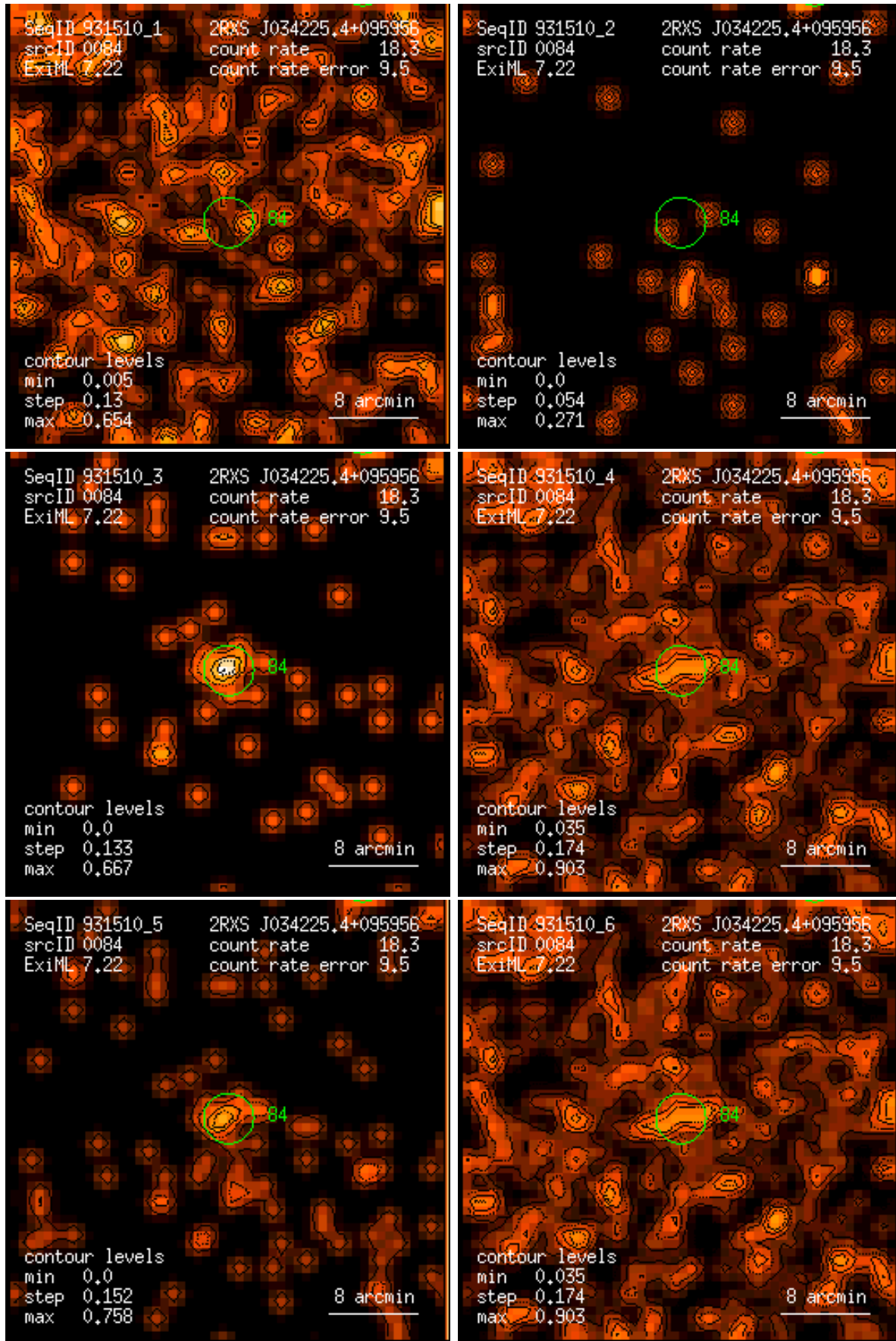
Figure 84: RASS 931510: detection 0084: band rate images, Gaussian filter: (1) PSPC channels 11 – 41, (2) 52 – 90, (3) 91 – 201, (4) 11 – 235, (5) 52 – 201, (6) 11 – 201. Broad band rates in counts/ks. Band rate contour levels in counts/ks/arcmin 2 .
