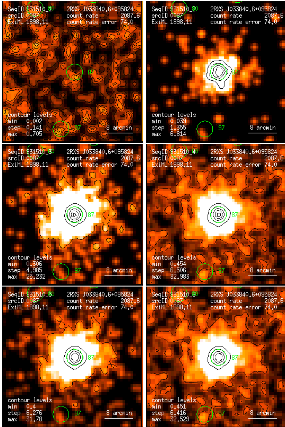
Figure 87: RASS 931510: detection 0087: band rate images, Gaussian filter: (1) PSPC channels 11 – 41, (2) 52 – 90, (3) 91 – 201, (4) 11 – 235, (5) 52 – 201, (6) 11 – 201. Broad band rates in counts/ks. Band rate contour levels in counts/ks/arcmin 2 .
