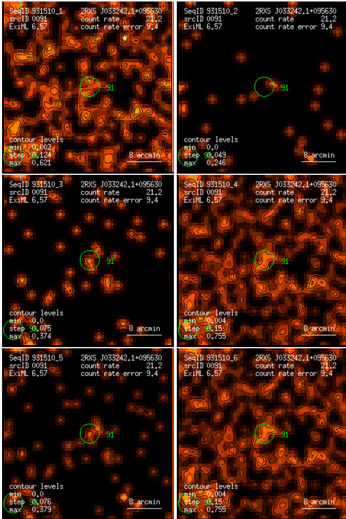
Figure 91: RASS 931510: detection 0091: band rate images, Gaussian filter: (1) PSPC channels 11 – 41, (2) 52 – 90, (3) 91 – 201, (4) 11 – 235, (5) 52 – 201, (6) 11 – 201. Broad band rates in counts/ks. Band rate contour levels in counts/ks/arcmin 2 .
