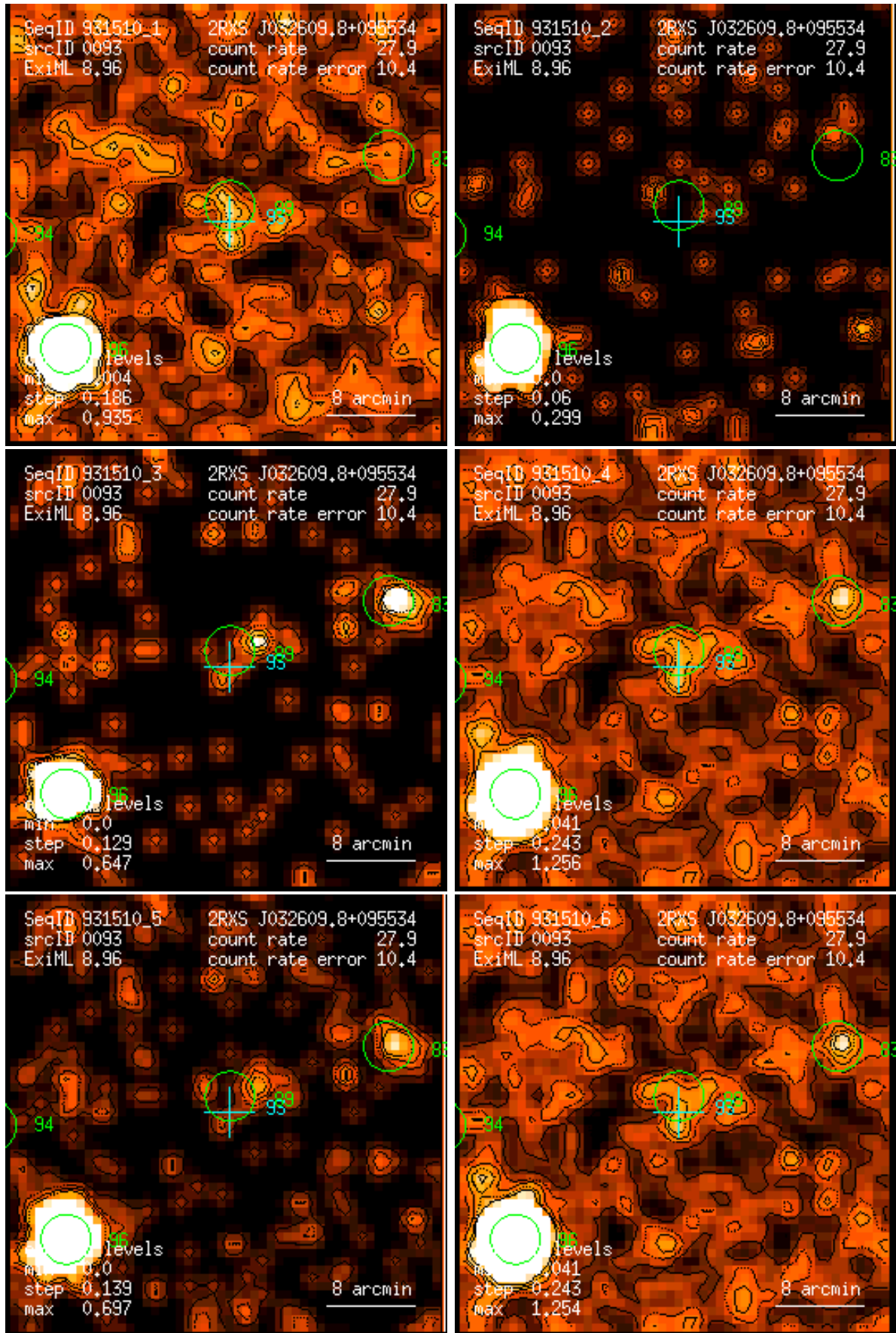
Figure 93: RASS 931510: detection 0093: band rate images, Gaussian filter: (1) PSPC channels 11 – 41, (2) 52 – 90, (3) 91 – 201, (4) 11 – 235, (5) 52 – 201, (6) 11 – 201. Broad band rates in counts/ks. Band rate contour levels in counts/ks/arcmin 2 .
