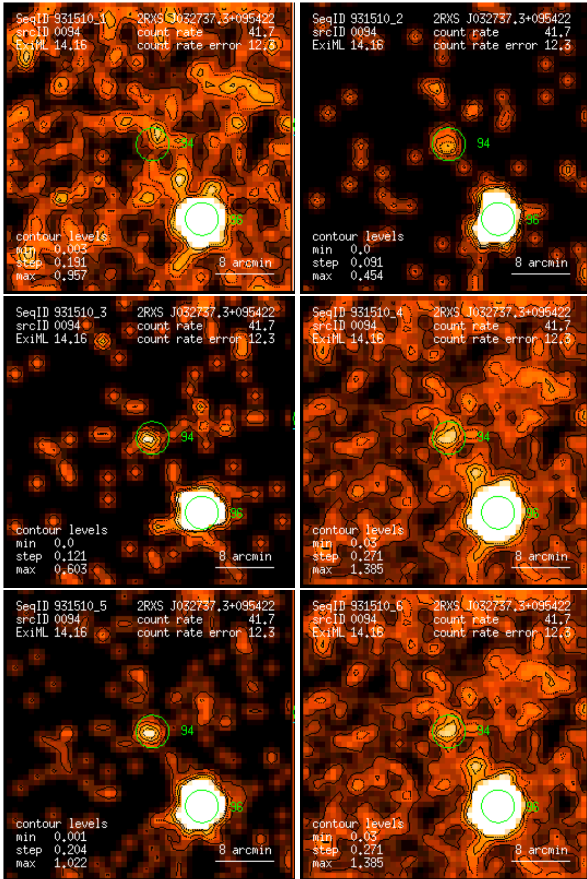
Figure 94: RASS 931510: detection 0094: band rate images, Gaussian filter: (1) PSPC channels 11 – 41, (2) 52 – 90, (3) 91 – 201, (4) 11 – 235, (5) 52 – 201, (6) 11 – 201. Broad band rates in counts/ks. Band rate contour levels in counts/ks/arcmin 2 .
