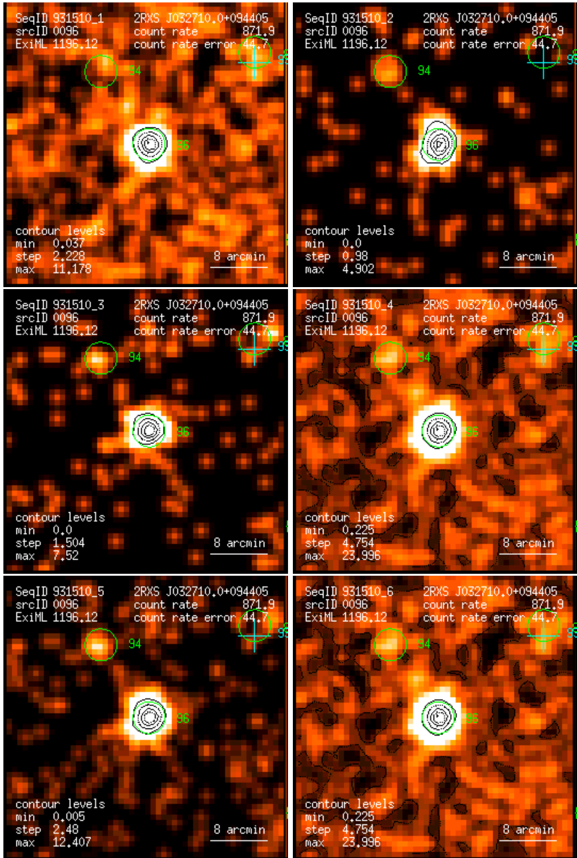
Figure 96: RASS 931510: detection 0096: band rate images, Gaussian filter: (1) PSPC channels 11 – 41, (2) 52 – 90, (3) 91 – 201, (4) 11 – 235, (5) 52 – 201, (6) 11 – 201. Broad band rates in counts/ks. Band rate contour levels in counts/ks/arcmin 2 .
