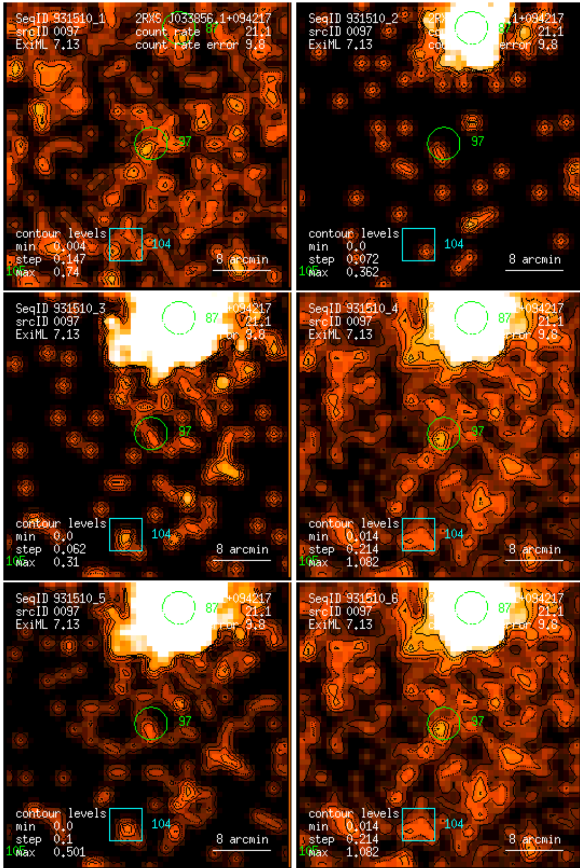
Figure 97: RASS 931510: detection 0097: band rate images, Gaussian filter: (1) PSPC channels 11 – 41, (2) 52 – 90, (3) 91 – 201, (4) 11 – 235, (5) 52 – 201, (6) 11 – 201. Broad band rates in counts/ks. Band rate contour levels in counts/ks/arcmin 2 .
