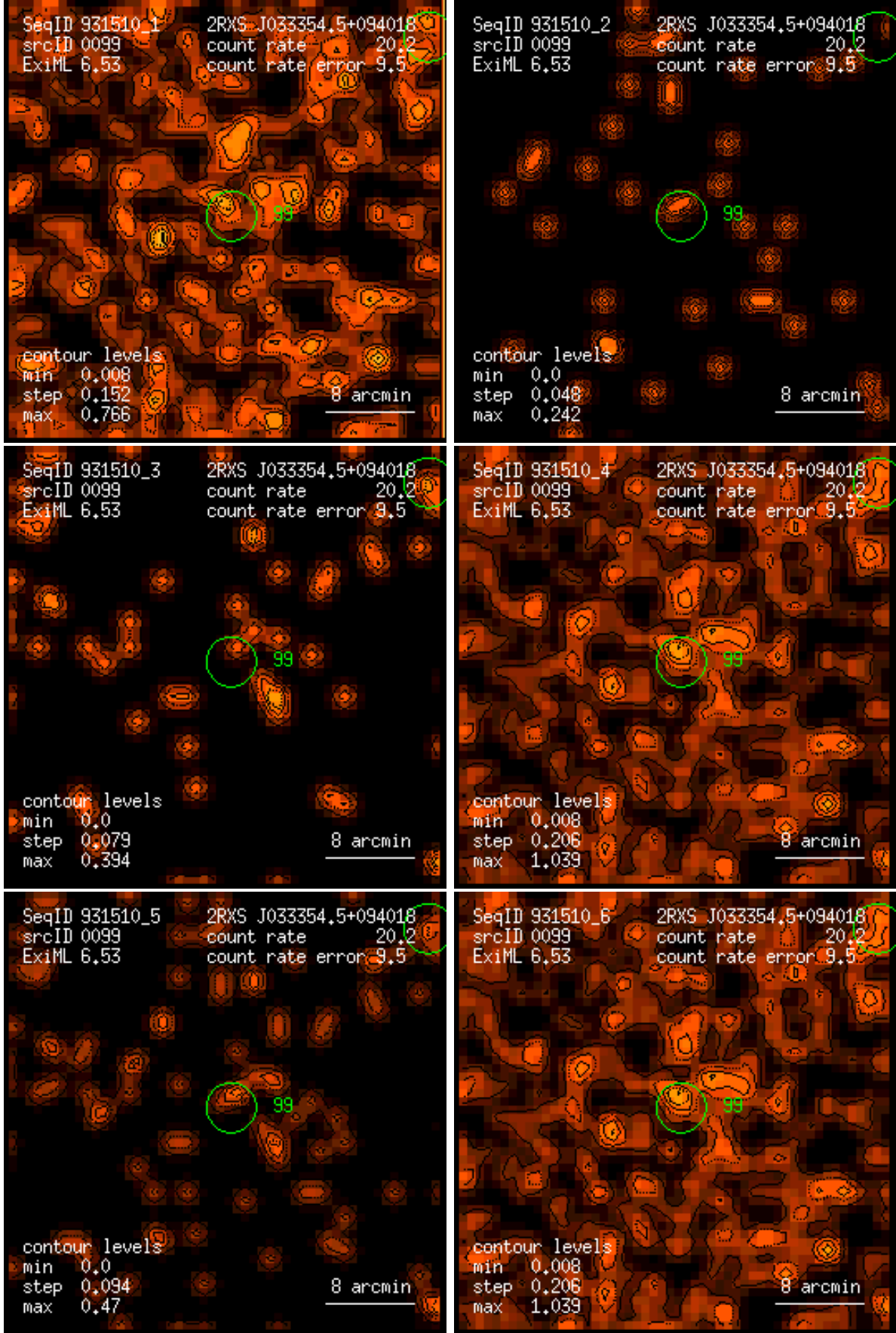
Figure 99: RASS 931510: detection 0099: band rate images, Gaussian filter: (1) PSPC channels 11 – 41, (2) 52 – 90, (3) 91 – 201, (4) 11 – 235, (5) 52 – 201, (6) 11 – 201. Broad band rates in counts/ks. Band rate contour levels in counts/ks/arcmin 2 .
