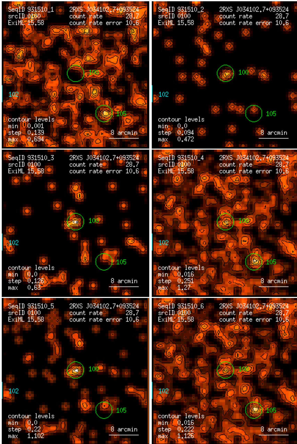
Figure 100: RASS 931510: detection 0100: band rate images, Gaussian filter: (1) PSPC channels 11 – 41, (2) 52 – 90, (3) 91 – 201, (4) 11 – 235, (5) 52 – 201, (6) 11 – 201. Broad band rates in counts/ks. Band rate contour levels in counts/ks/arcmin 2 .
