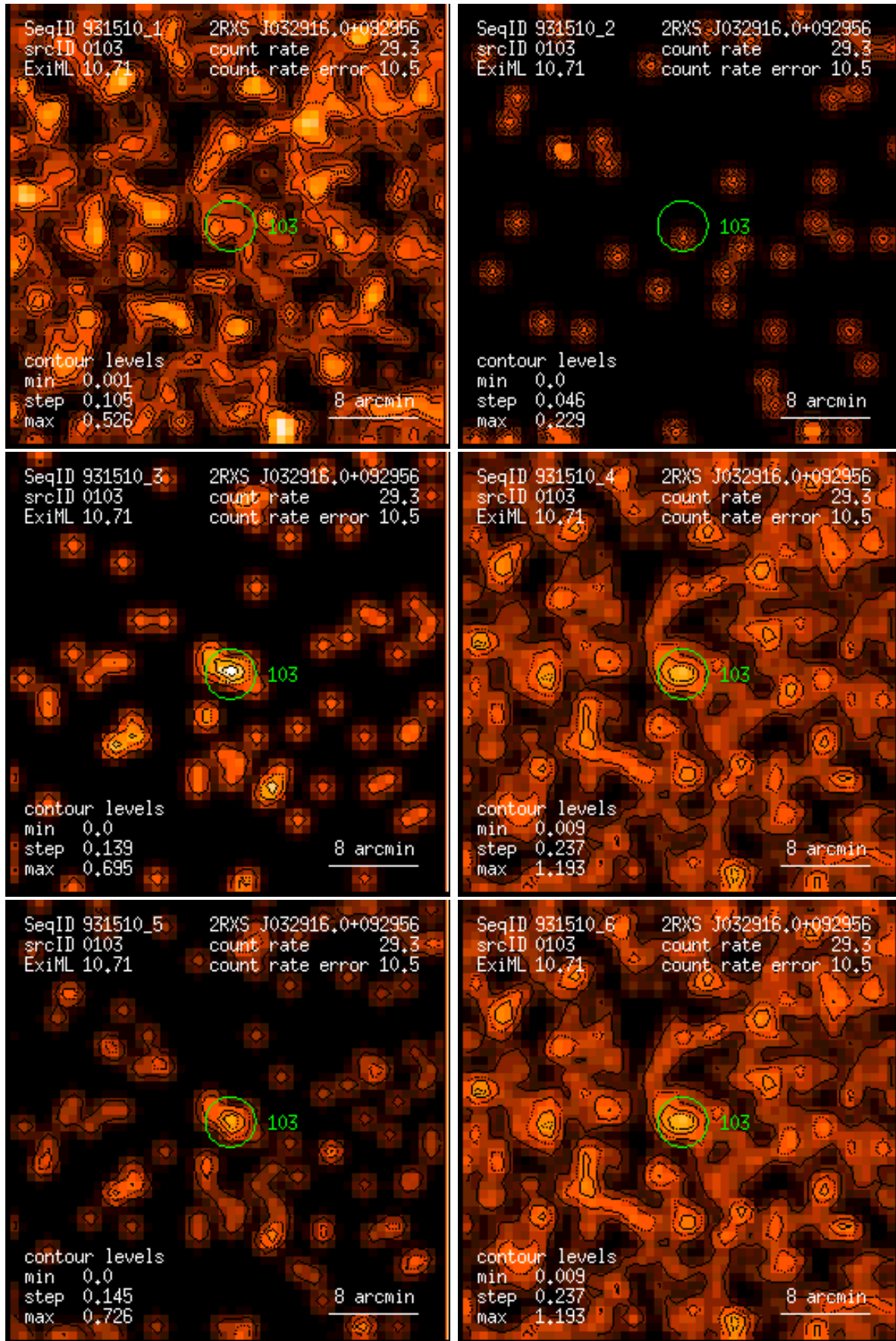
Figure 103: RASS 931510: detection 0103: band rate images, Gaussian filter: (1) PSPC channels 11 – 41, (2) 52 – 90, (3) 91 – 201, (4) 11 – 235, (5) 52 – 201, (6) 11 – 201. Broad band rates in counts/ks. Band rate contour levels in counts/ks/arcmin 2 .
