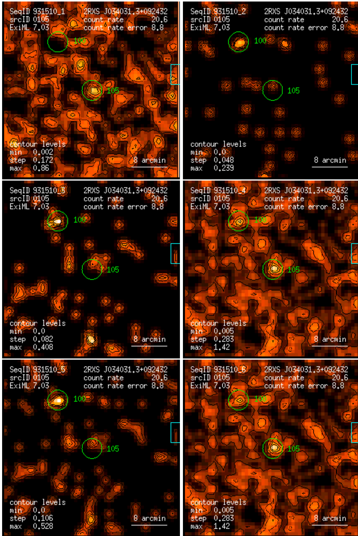
Figure 105: RASS 931510: detection 0105: band rate images, Gaussian filter: (1) PSPC channels 11 – 41, (2) 52 – 90, (3) 91 – 201, (4) 11 – 235, (5) 52 – 201, (6) 11 – 201. Broad band rates in counts/ks. Band rate contour levels in counts/ks/arcmin 2 .
