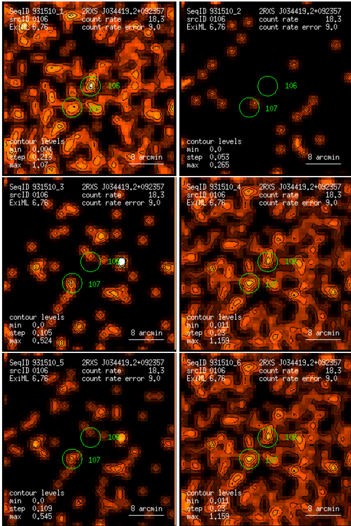
Figure 106: RASS 931510: detection 0106: band rate images, Gaussian filter: (1) PSPC channels 11 – 41, (2) 52 – 90, (3) 91 – 201, (4) 11 – 235, (5) 52 – 201, (6) 11 – 201. Broad band rates in counts/ks. Band rate contour levels in counts/ks/arcmin 2 .
