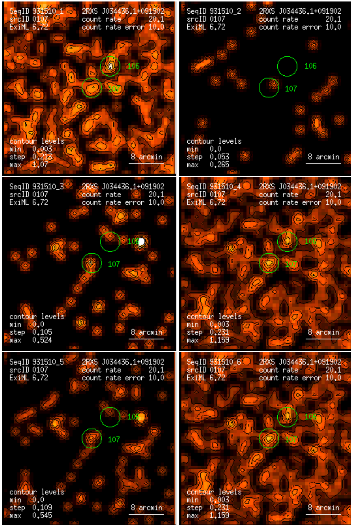
Figure 107: RASS 931510: detection 0107: band rate images, Gaussian filter: (1) PSPC channels 11 – 41, (2) 52 – 90, (3) 91 – 201, (4) 11 – 235, (5) 52 – 201, (6) 11 – 201. Broad band rates in counts/ks. Band rate contour levels in counts/ks/arcmin 2 .
